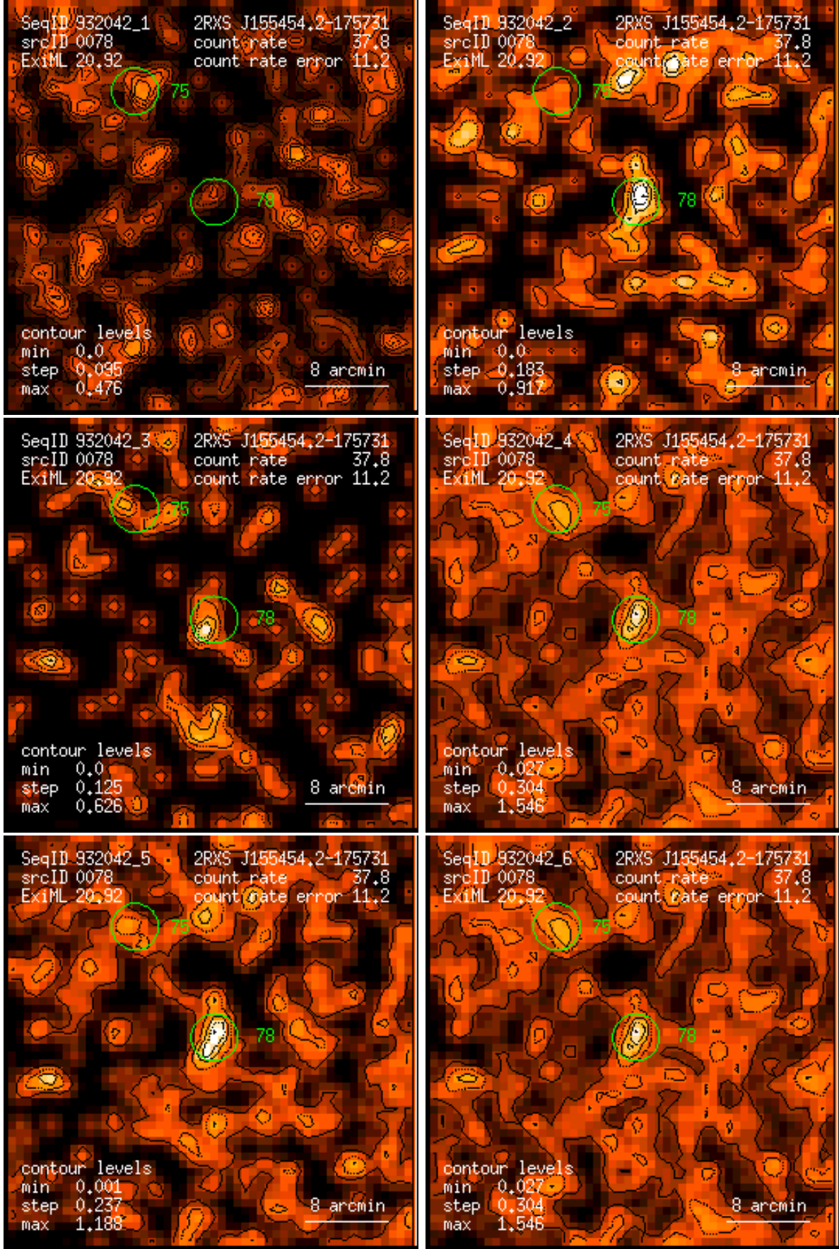
Figure 78: RASS 932042: detection 0078: band rate images, Gaussian filter: (1) PSPC channels 11 – 41, (2) 52 – 90, (3) 91 – 201, (4) 11 – 235, (5) 52 – 201, (6) 11 – 201. Broad band rates in counts/ks. Band rate contour levels in counts/ks/arcmin 2 .
