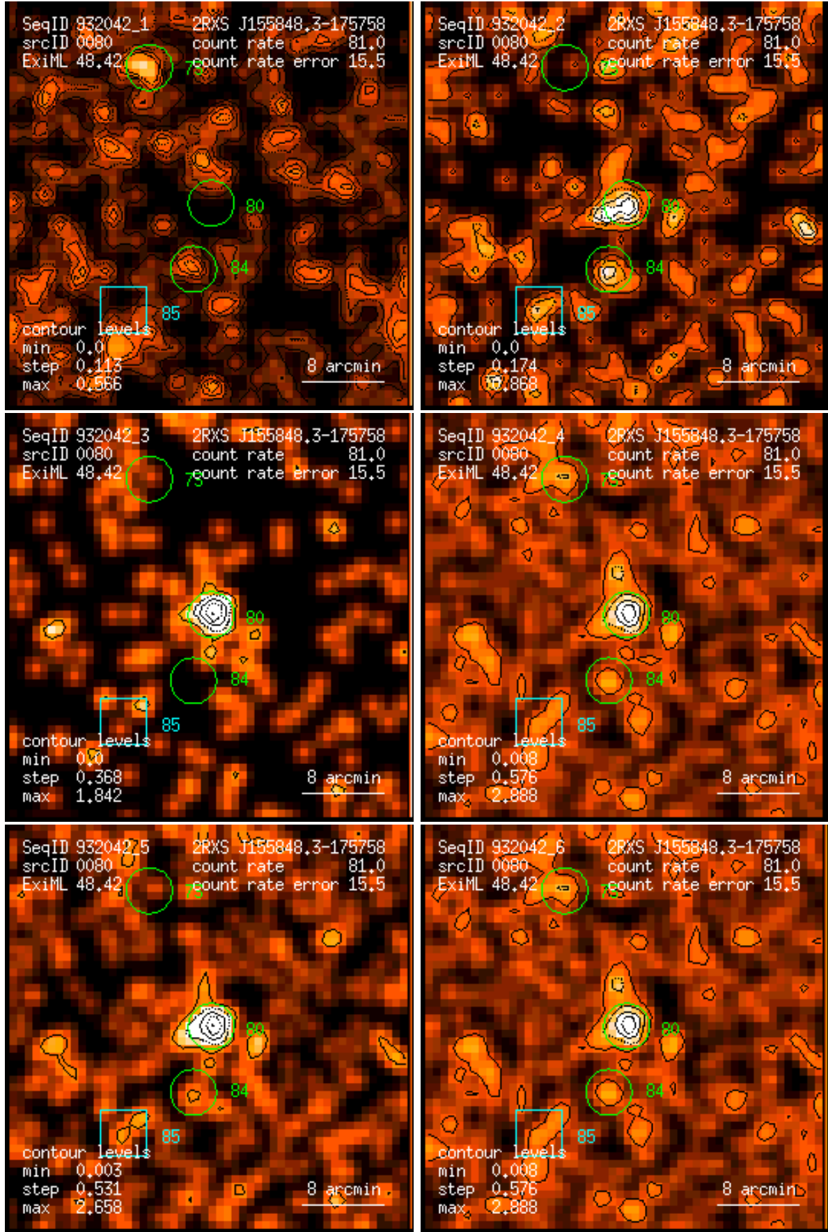
Figure 80: RASS 932042: detection 0080: band rate images, Gaussian filter: (1) PSPC channels 11 – 41, (2) 52 – 90, (3) 91 – 201, (4) 11 – 235, (5) 52 – 201, (6) 11 – 201. Broad band rates in counts/ks. Band rate contour levels in counts/ks/arcmin 2 .
