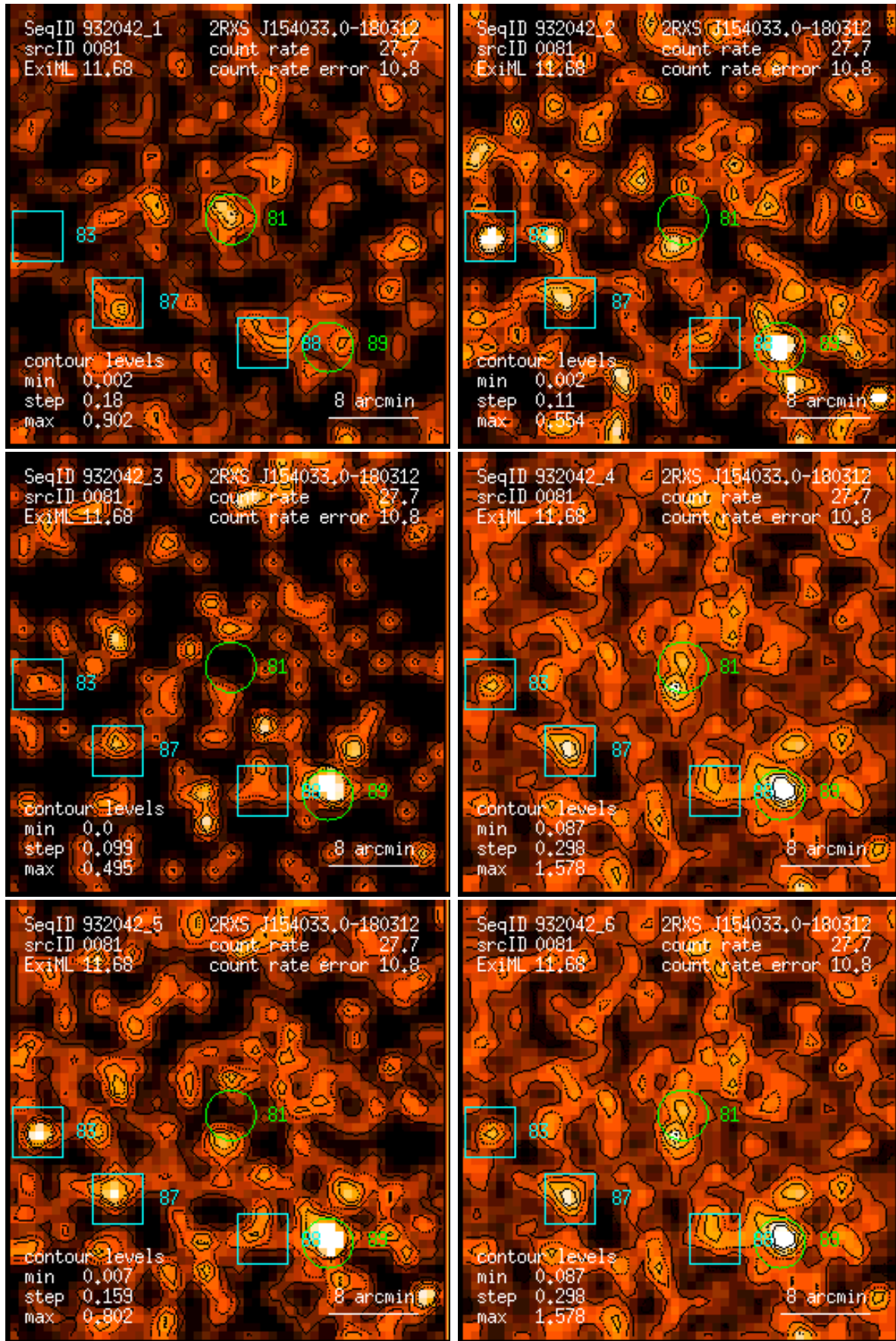
Figure 81: RASS 932042: detection 0081: band rate images, Gaussian filter: (1) PSPC channels 11 – 41, (2) 52 – 90, (3) 91 – 201, (4) 11 – 235, (5) 52 – 201, (6) 11 – 201. Broad band rates in counts/ks. Band rate contour levels in counts/ks/arcmin 2 .
