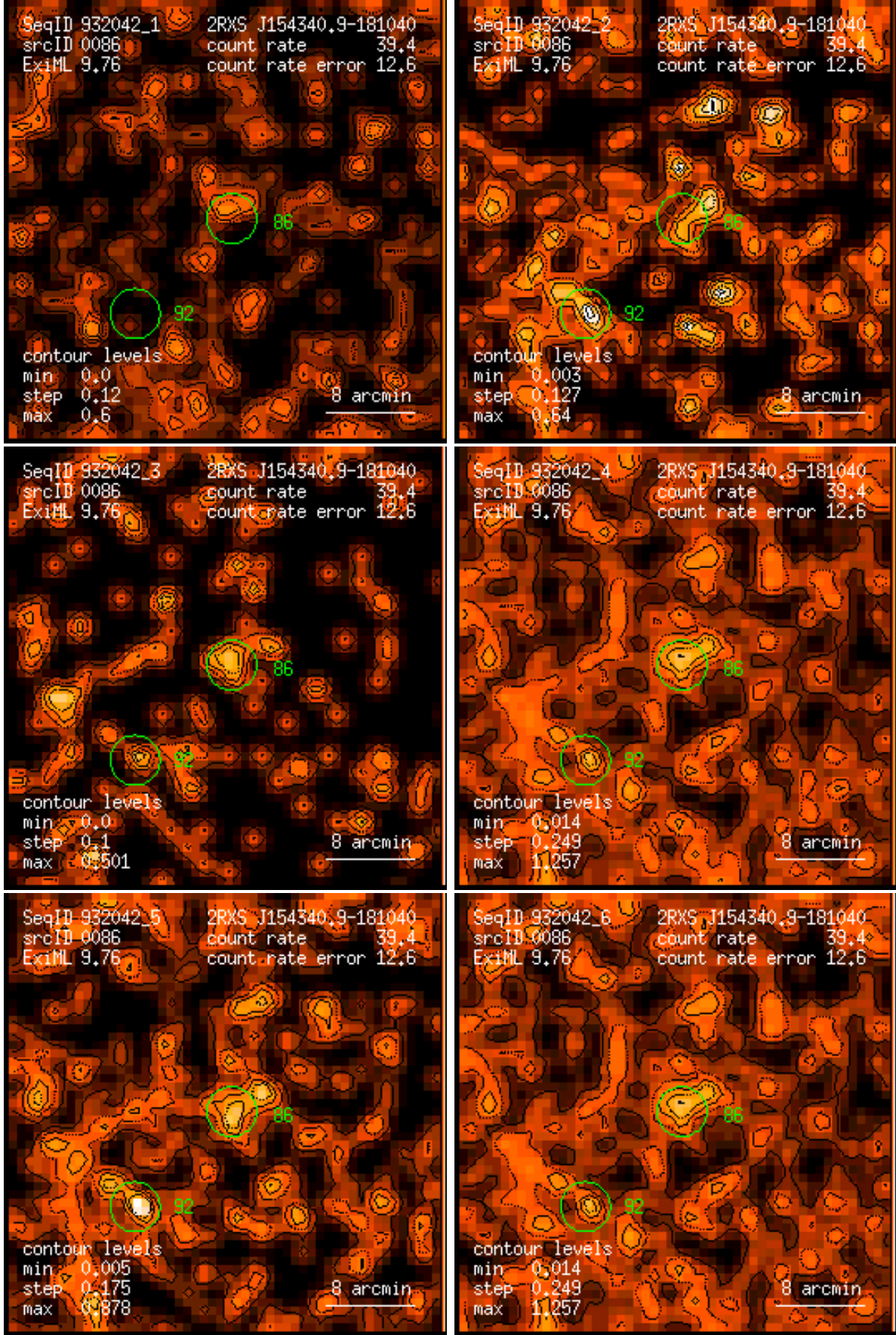
Figure 86: RASS 932042: detection 0086: band rate images, Gaussian filter: (1) PSPC channels 11 – 41, (2) 52 – 90, (3) 91 – 201, (4) 11 – 235, (5) 52 – 201, (6) 11 – 201. Broad band rates in counts/ks. Band rate contour levels in counts/ks/arcmin 2 .
