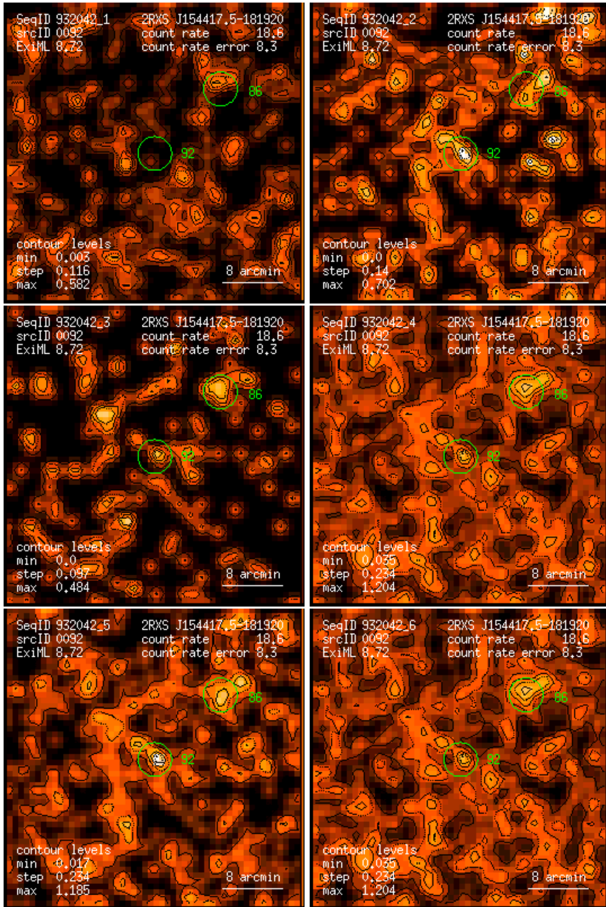
Figure 92: RASS 932042: detection 0092: band rate images, Gaussian filter: (1) PSPC channels 11 – 41, (2) 52 – 90, (3) 91 – 201, (4) 11 – 235, (5) 52 – 201, (6) 11 – 201. Broad band rates in counts/ks. Band rate contour levels in counts/ks/arcmin 2 .
