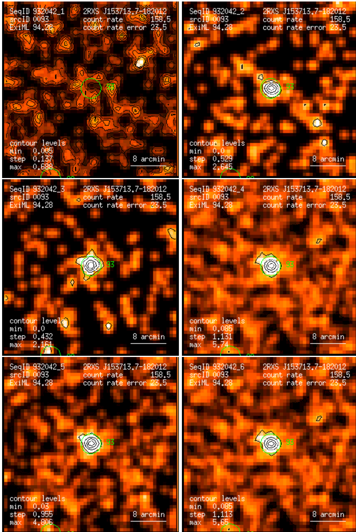
Figure 93: RASS 932042: detection 0093: band rate images, Gaussian filter: (1) PSPC channels 11 – 41, (2) 52 – 90, (3) 91 – 201, (4) 11 – 235, (5) 52 – 201, (6) 11 – 201. Broad band rates in counts/ks. Band rate contour levels in counts/ks/arcmin 2 .
