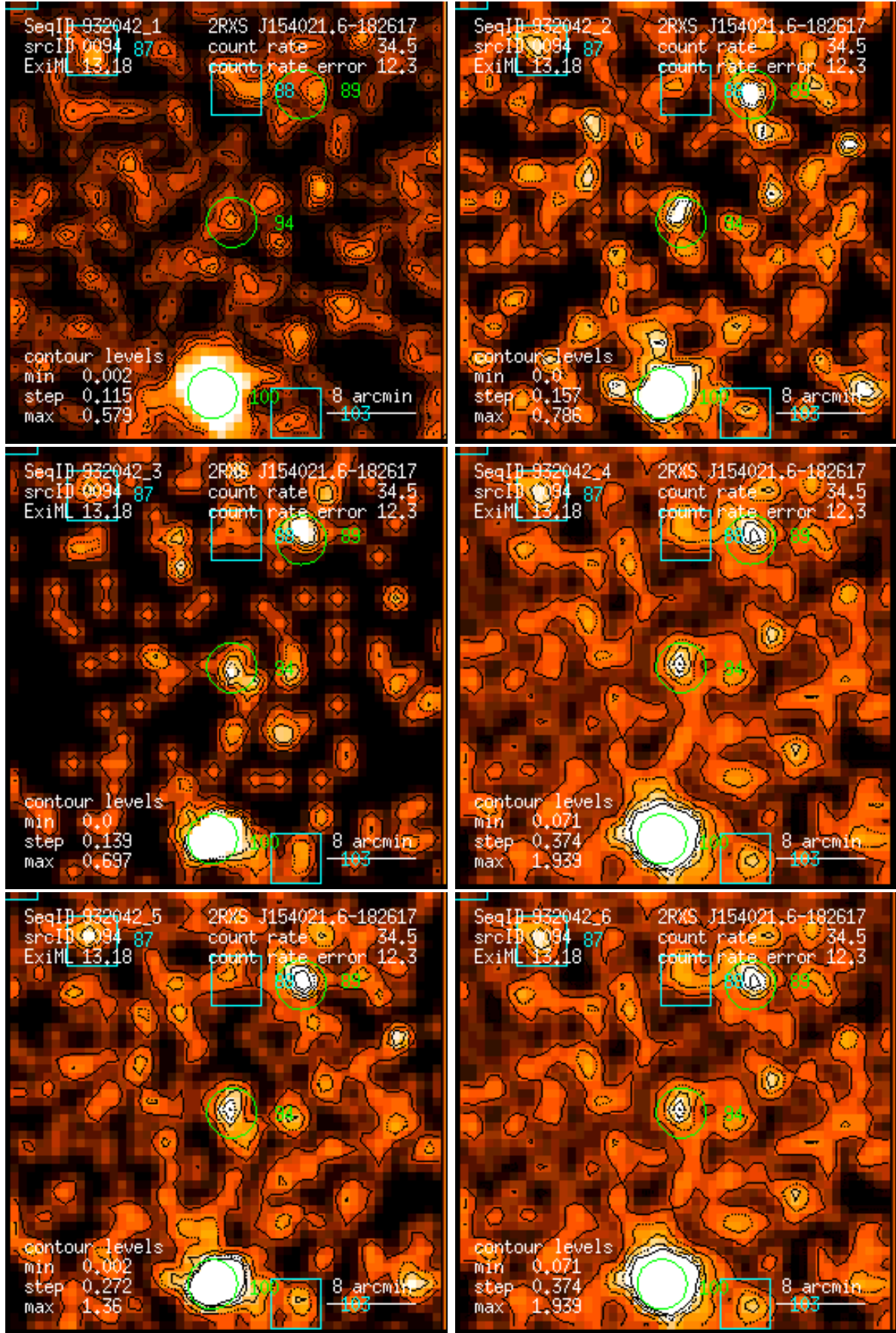
Figure 94: RASS 932042: detection 0094: band rate images, Gaussian filter: (1) PSPC channels 11 – 41, (2) 52 – 90, (3) 91 – 201, (4) 11 – 235, (5) 52 – 201, (6) 11 – 201. Broad band rates in counts/ks. Band rate contour levels in counts/ks/arcmin 2 .
