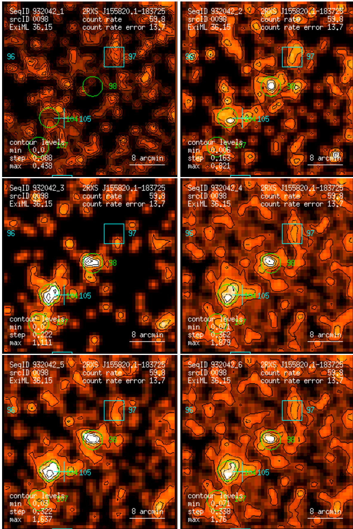
Figure 98: RASS 932042: detection 0098: band rate images, Gaussian filter: (1) PSPC channels 11 – 41, (2) 52 – 90, (3) 91 – 201, (4) 11 – 235, (5) 52 – 201, (6) 11 – 201. Broad band rates in counts/ks. Band rate contour levels in counts/ks/arcmin 2 .
