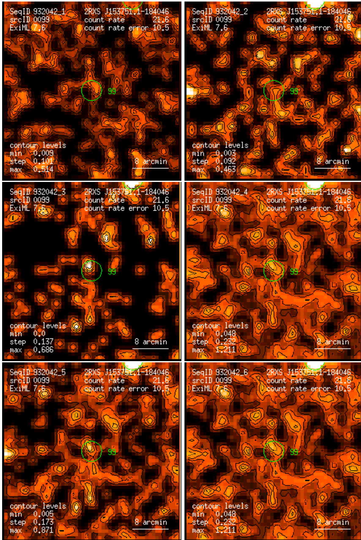
Figure 99: RASS 932042: detection 0099: band rate images, Gaussian filter: (1) PSPC channels 11 – 41, (2) 52 – 90, (3) 91 – 201, (4) 11 – 235, (5) 52 – 201, (6) 11 – 201. Broad band rates in counts/ks. Band rate contour levels in counts/ks/arcmin 2 .
