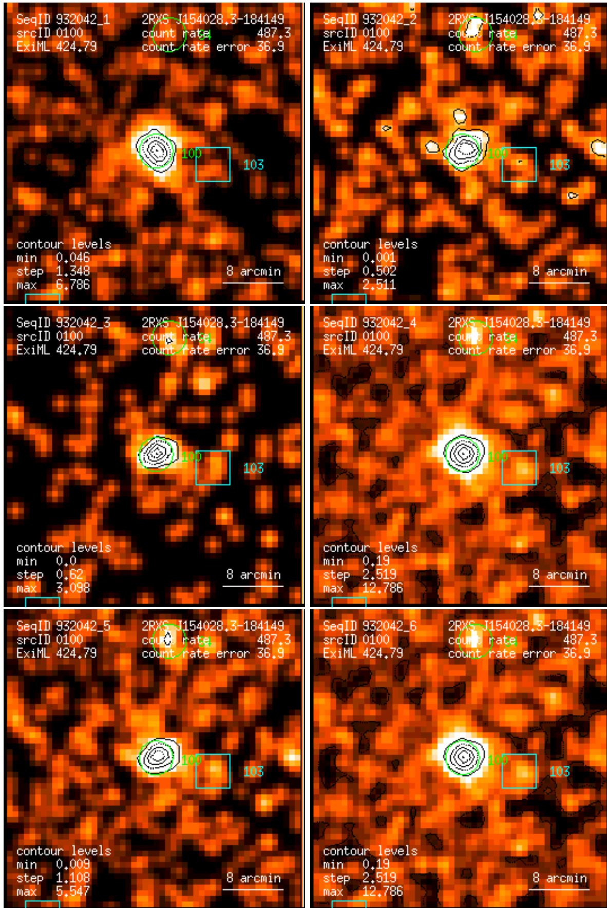
Figure 100: RASS 932042: detection 0100: band rate images, Gaussian filter: (1) PSPC channels 11 – 41, (2) 52 – 90, (3) 91 – 201, (4) 11 – 235, (5) 52 – 201, (6) 11 – 201. Broad band rates in counts/ks. Band rate contour levels in counts/ks/arcmin 2 .
