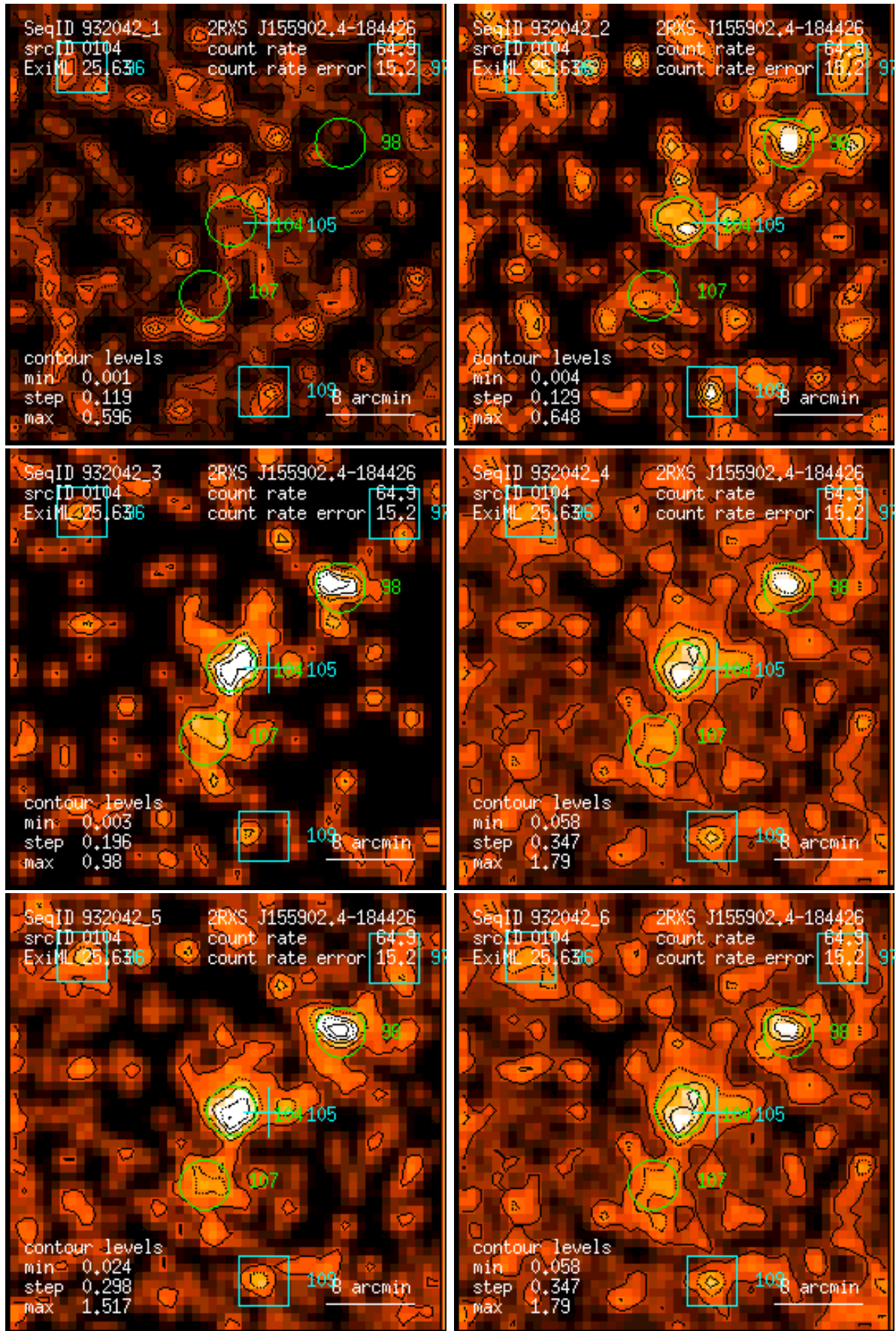
Figure 104: RASS 932042: detection 0104: band rate images, Gaussian filter: (1) PSPC channels 11 – 41, (2) 52 – 90, (3) 91 – 201, (4) 11 – 235, (5) 52 – 201, (6) 11 – 201. Broad band rates in counts/ks. Band rate contour levels in counts/ks/arcmin 2 .
