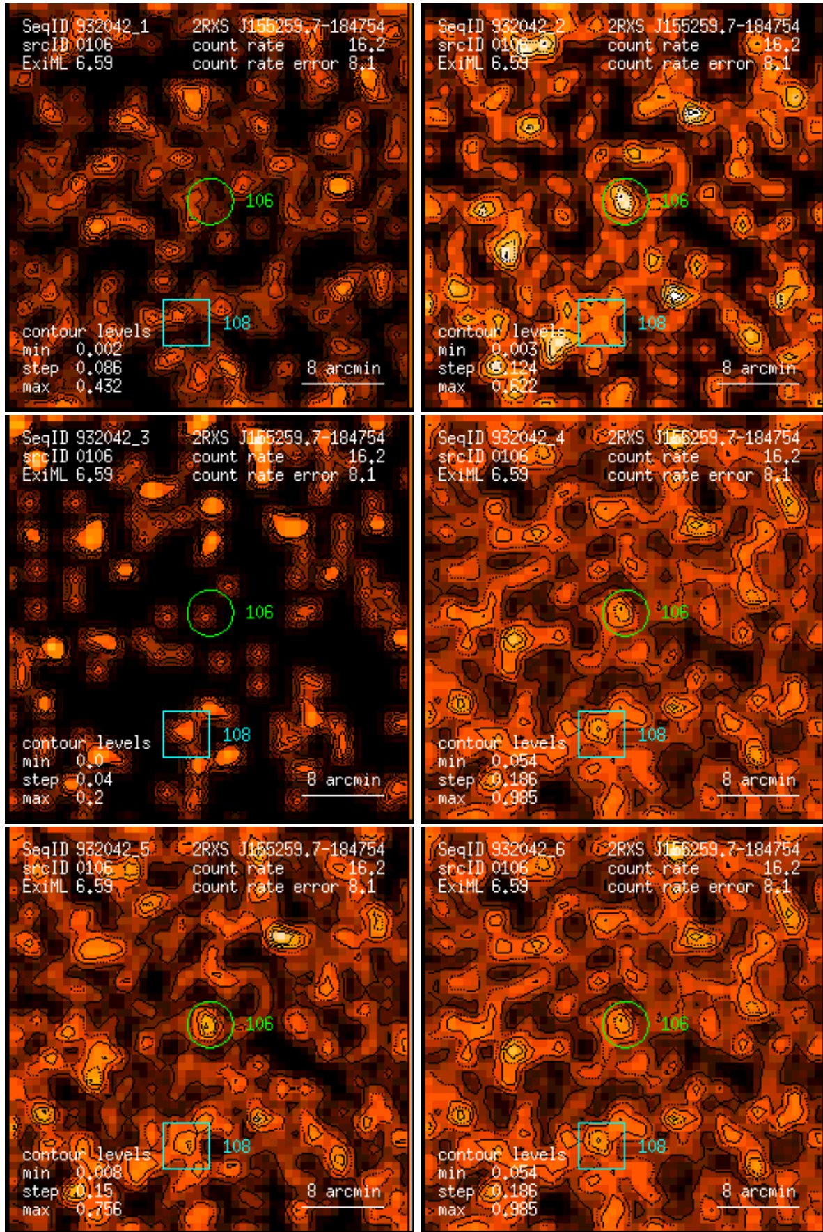
Figure 106: RASS 932042: detection 0106: band rate images, Gaussian filter: (1) PSPC channels 11 – 41, (2) 52 – 90, (3) 91 – 201, (4) 11 – 235, (5) 52 – 201, (6) 11 – 201. Broad band rates in counts/ks. Band rate contour levels in counts/ks/arcmin 2 .
