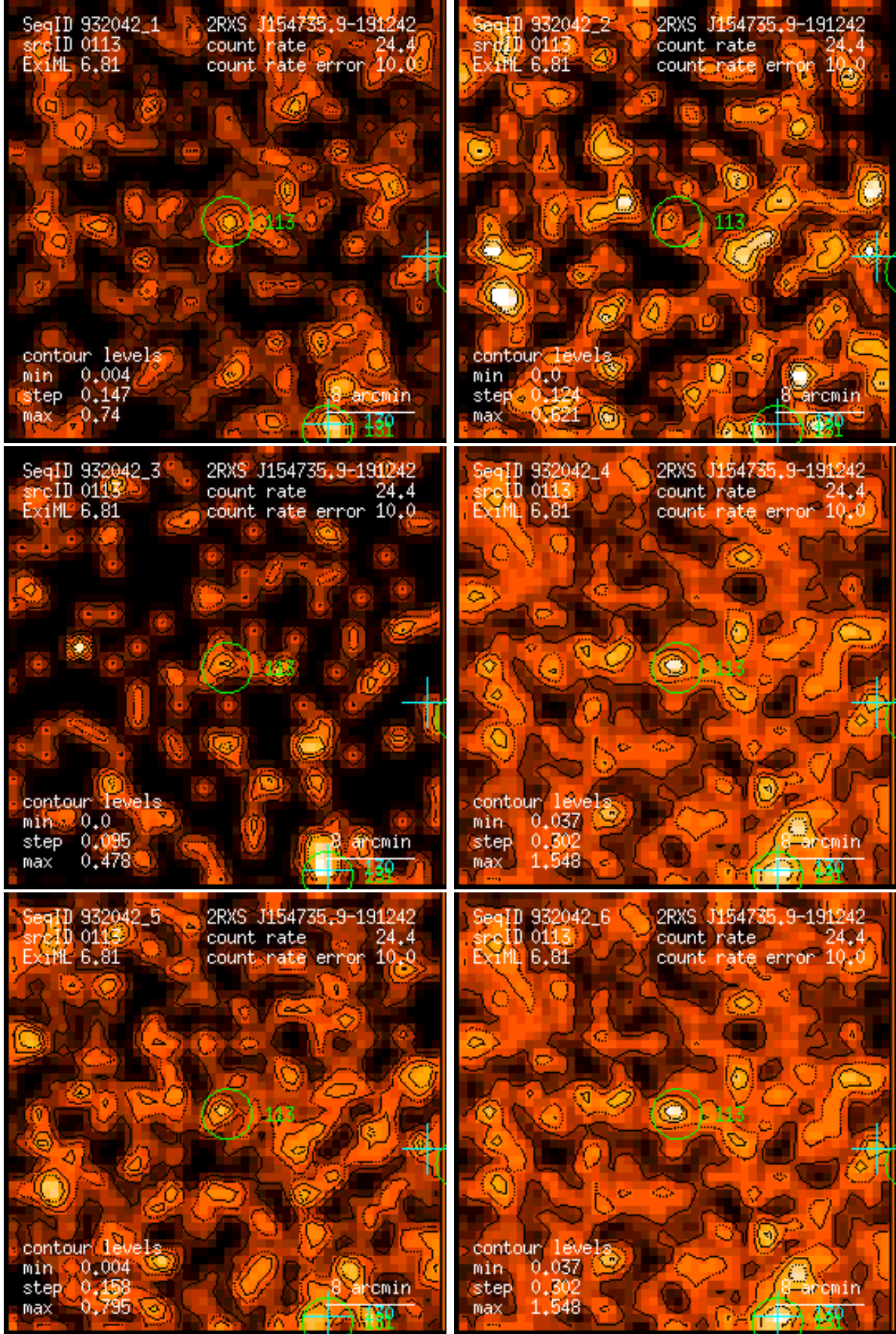
Figure 113: RASS 932042: detection 0113: band rate images, Gaussian filter: (1) PSPC channels 11 – 41, (2) 52 – 90, (3) 91 – 201, (4) 11 – 235, (5) 52 – 201, (6) 11 – 201. Broad band rates in counts/ks. Band rate contour levels in counts/ks/arcmin 2 .
