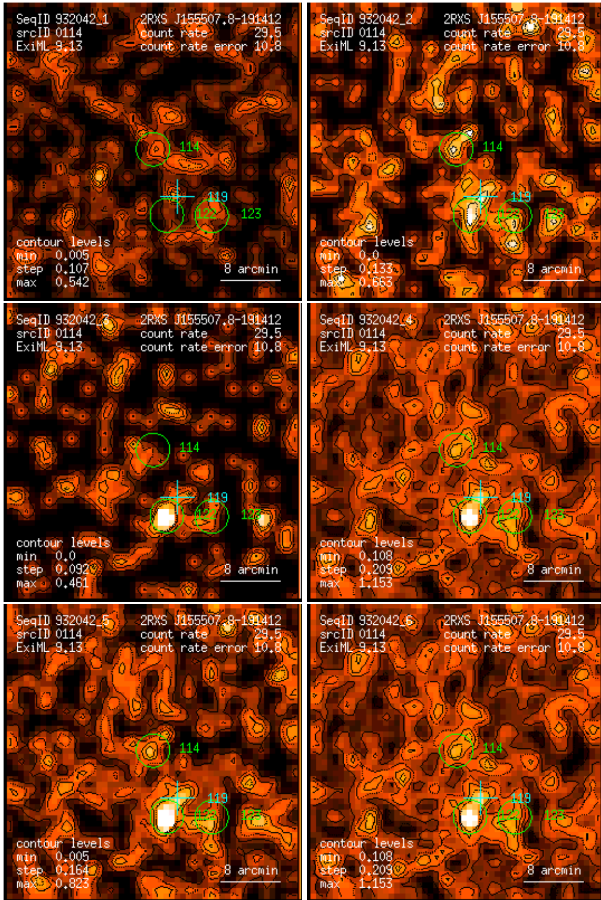
Figure 114: RASS 932042: detection 0114: band rate images, Gaussian filter: (1) PSPC channels 11 – 41, (2) 52 – 90, (3) 91 – 201, (4) 11 – 235, (5) 52 – 201, (6) 11 – 201. Broad band rates in counts/ks. Band rate contour levels in counts/ks/arcmin 2 .
