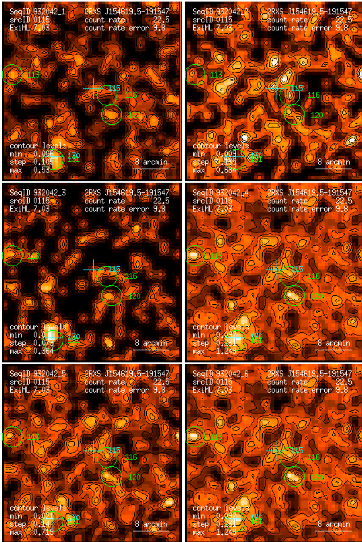
Figure 115: RASS 932042: detection 0115: band rate images, Gaussian filter: (1) PSPC channels 11 – 41, (2) 52 – 90, (3) 91 – 201, (4) 11 – 235, (5) 52 – 201, (6) 11 – 201. Broad band rates in counts/ks. Band rate contour levels in counts/ks/arcmin 2 .
