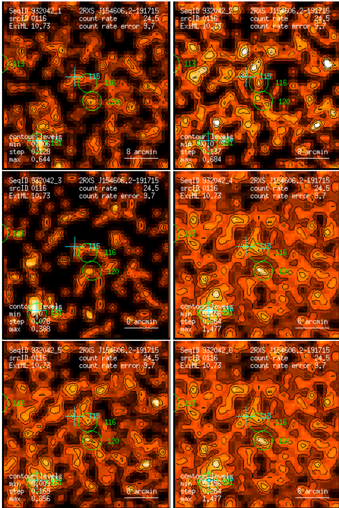
Figure 116: RASS 932042: detection 0116: band rate images, Gaussian filter: (1) PSPC channels 11 – 41, (2) 52 – 90, (3) 91 – 201, (4) 11 – 235, (5) 52 – 201, (6) 11 – 201. Broad band rates in counts/ks. Band rate contour levels in counts/ks/arcmin 2 .
