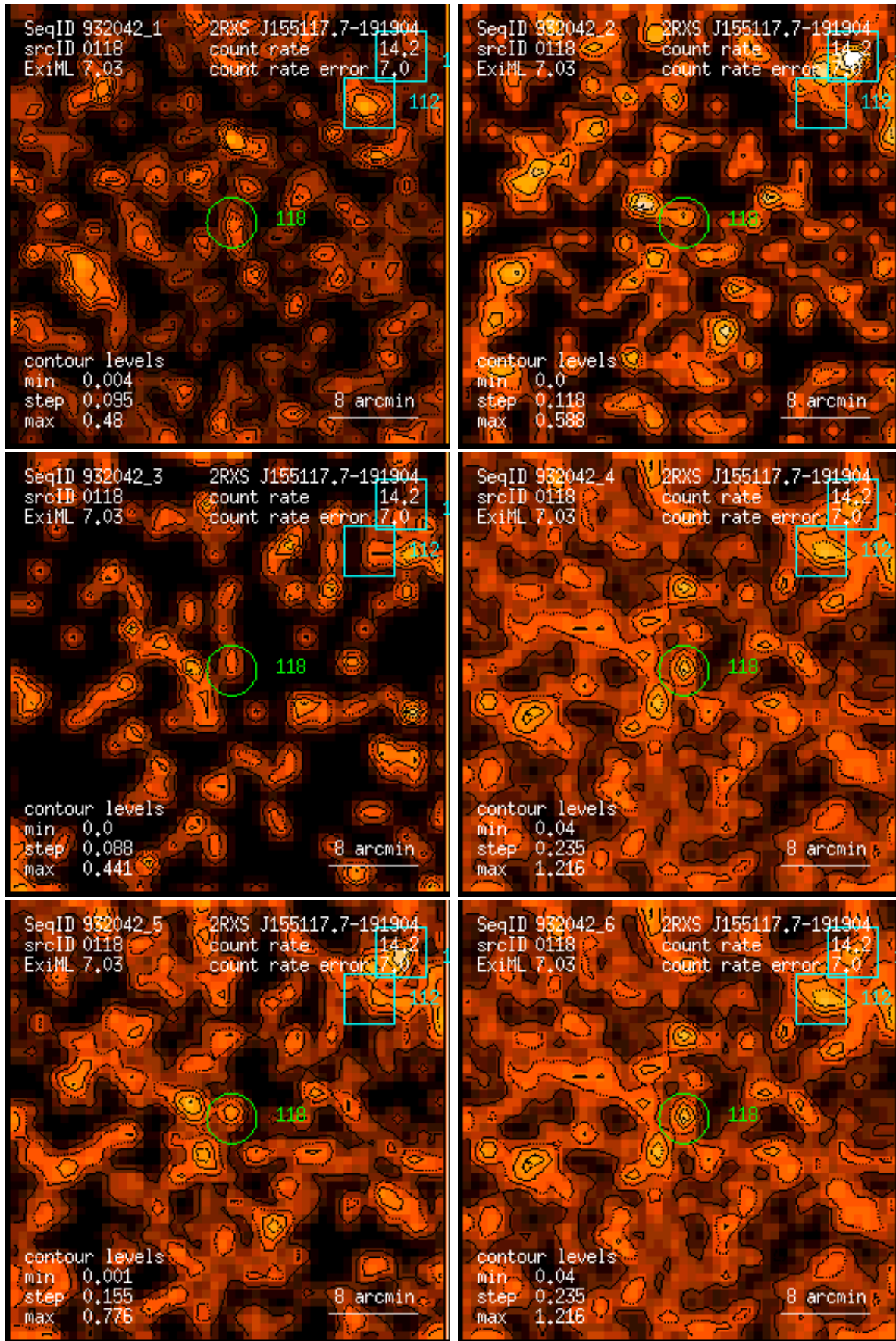
Figure 118: RASS 932042: detection 0118: band rate images, Gaussian filter: (1) PSPC channels 11 – 41, (2) 52 – 90, (3) 91 – 201, (4) 11 – 235, (5) 52 – 201, (6) 11 – 201. Broad band rates in counts/ks. Band rate contour levels in counts/ks/arcmin 2 .
