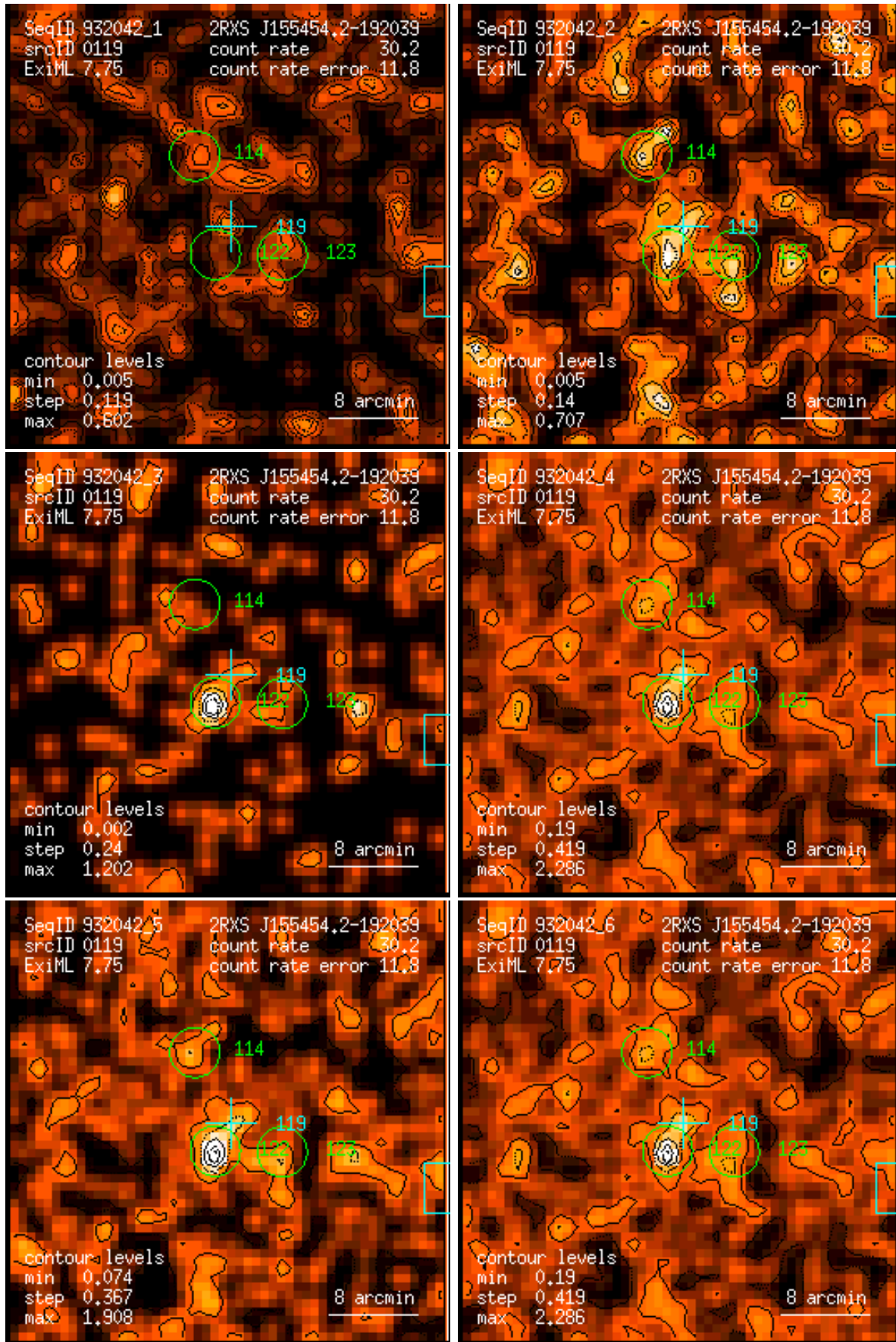
Figure 119: RASS 932042: detection 0119: band rate images, Gaussian filter: (1) PSPC channels 11 – 41, (2) 52 – 90, (3) 91 – 201, (4) 11 – 235, (5) 52 – 201, (6) 11 – 201. Broad band rates in counts/ks. Band rate contour levels in counts/ks/arcmin 2 .
