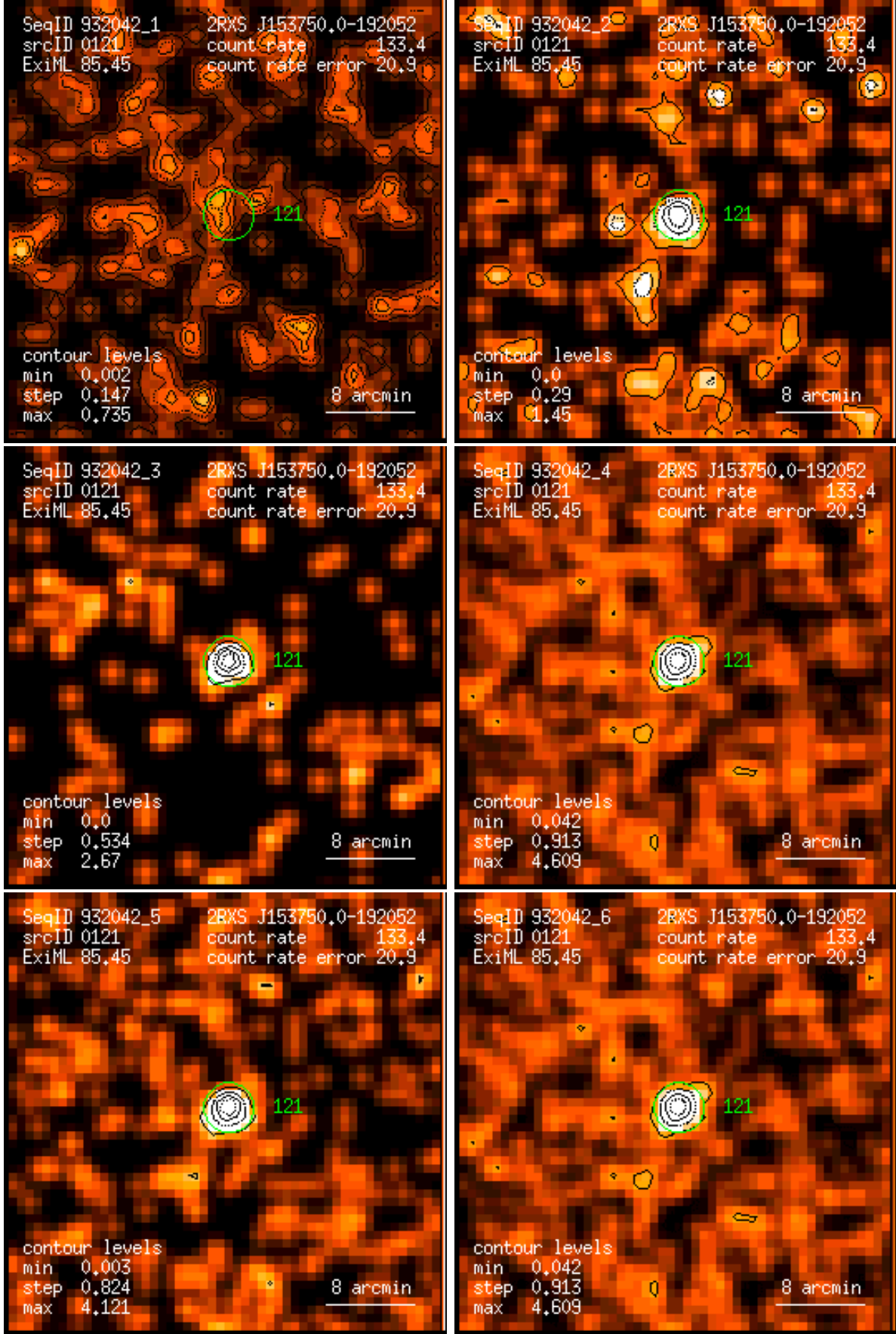
Figure 121: RASS 932042: detection 0121: band rate images, Gaussian filter: (1) PSPC channels 11 – 41, (2) 52 – 90, (3) 91 – 201, (4) 11 – 235, (5) 52 – 201, (6) 11 – 201. Broad band rates in counts/ks. Band rate contour levels in counts/ks/arcmin 2 .
