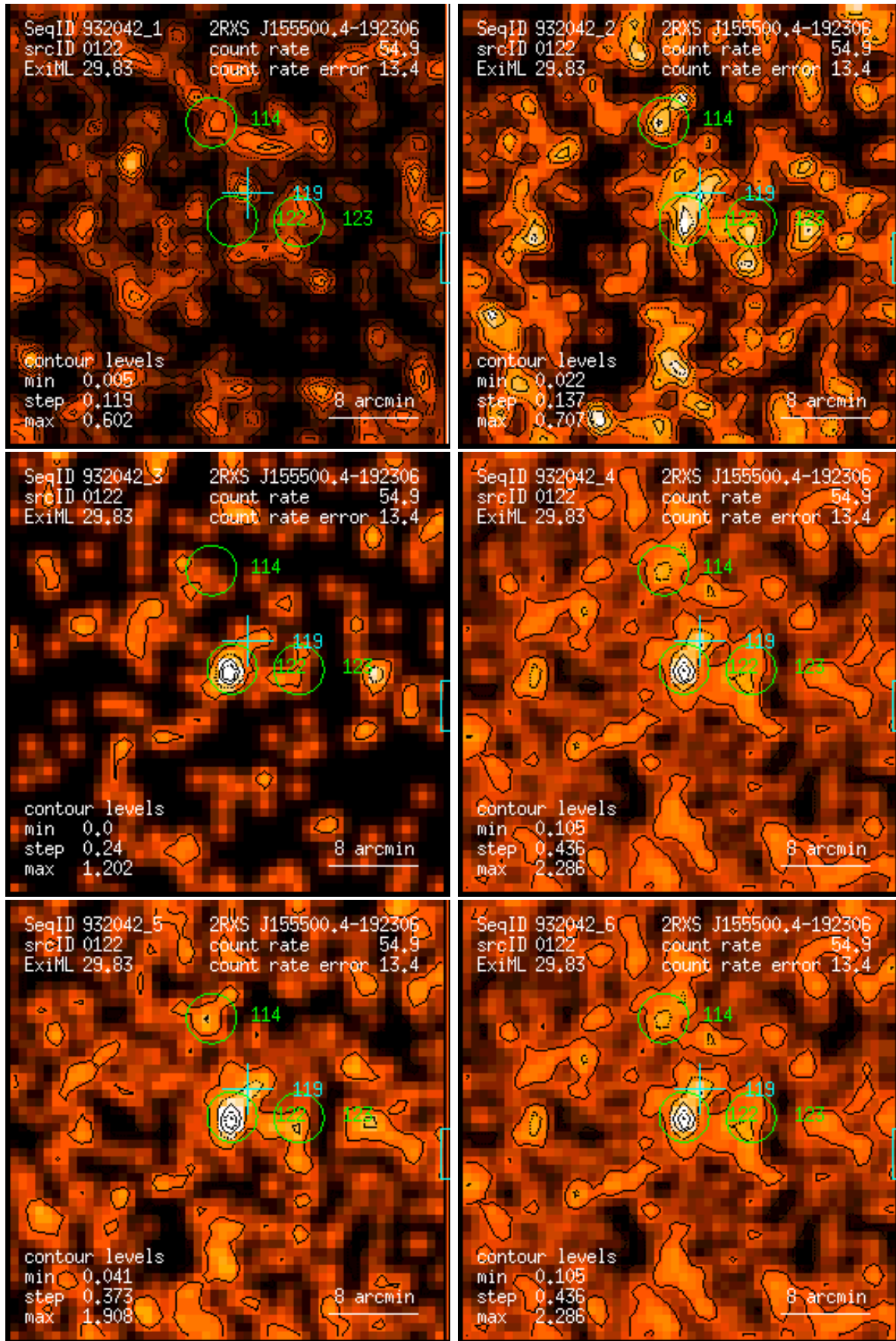
Figure 122: RASS 932042: detection 0122: band rate images, Gaussian filter: (1) PSPC channels 11 – 41, (2) 52 – 90, (3) 91 – 201, (4) 11 – 235, (5) 52 – 201, (6) 11 – 201. Broad band rates in counts/ks. Band rate contour levels in counts/ks/arcmin 2 .
