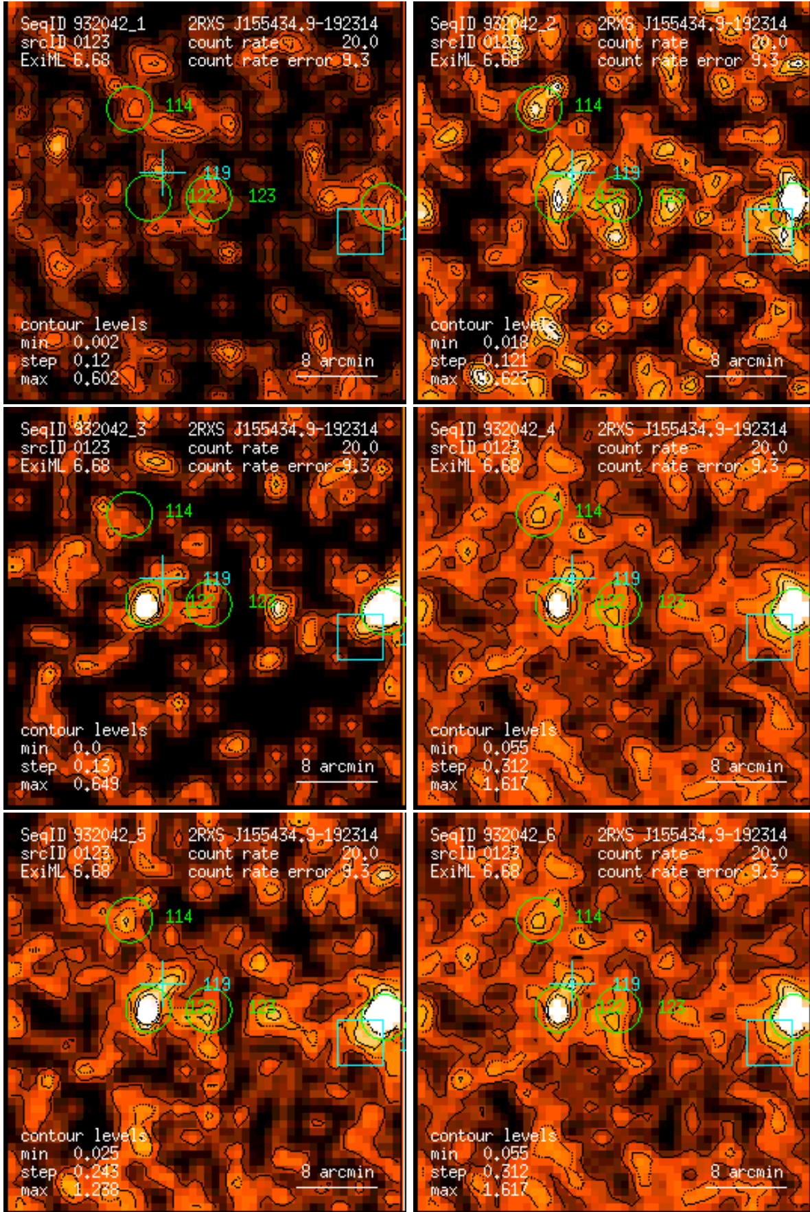
Figure 123: RASS 932042: detection 0123: band rate images, Gaussian filter: (1) PSPC channels 11 – 41, (2) 52 – 90, (3) 91 – 201, (4) 11 – 235, (5) 52 – 201, (6) 11 – 201. Broad band rates in counts/ks. Band rate contour levels in counts/ks/arcmin 2 .
