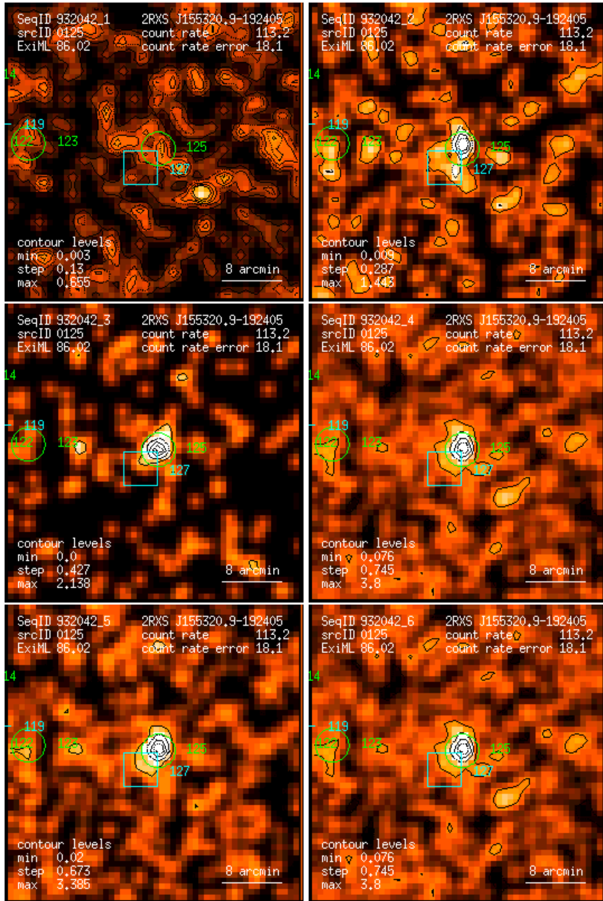
Figure 125: RASS 932042: detection 0125: band rate images, Gaussian filter: (1) PSPC channels 11 – 41, (2) 52 – 90, (3) 91 – 201, (4) 11 – 235, (5) 52 – 201, (6) 11 – 201. Broad band rates in counts/ks. Band rate contour levels in counts/ks/arcmin 2 .
