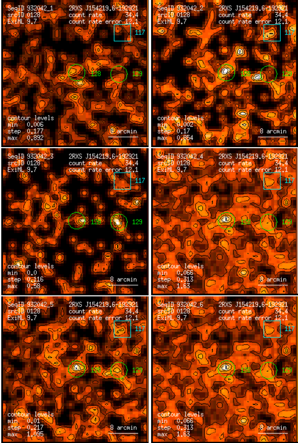
Figure 128: RASS 932042: detection 0128: band rate images, Gaussian filter: (1) PSPC channels 11 – 41, (2) 52 – 90, (3) 91 – 201, (4) 11 – 235, (5) 52 – 201, (6) 11 – 201. Broad band rates in counts/ks. Band rate contour levels in counts/ks/arcmin 2 .
