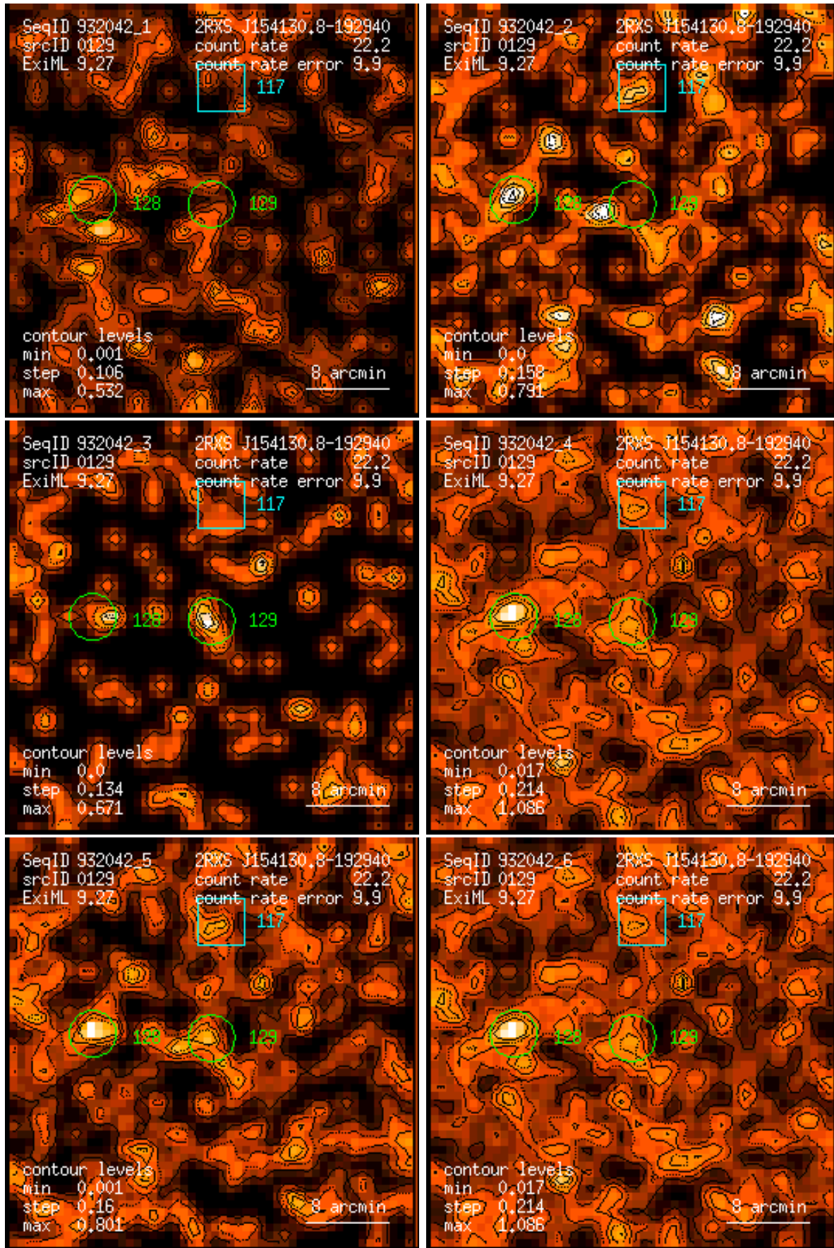
Figure 129: RASS 932042: detection 0129: band rate images, Gaussian filter: (1) PSPC channels 11 – 41, (2) 52 – 90, (3) 91 – 201, (4) 11 – 235, (5) 52 – 201, (6) 11 – 201. Broad band rates in counts/ks. Band rate contour levels in counts/ks/arcmin 2 .
