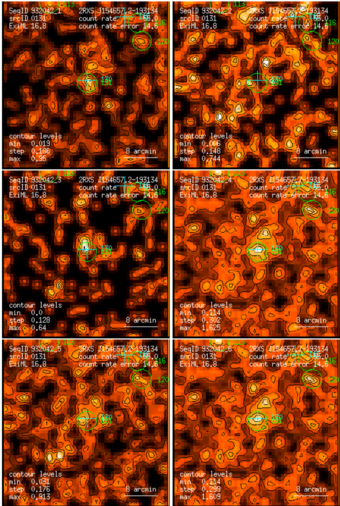
Figure 131: RASS 932042: detection 0131: band rate images, Gaussian filter: (1) PSPC channels 11 – 41, (2) 52 – 90, (3) 91 – 201, (4) 11 – 235, (5) 52 – 201, (6) 11 – 201. Broad band rates in counts/ks. Band rate contour levels in counts/ks/arcmin 2 .
