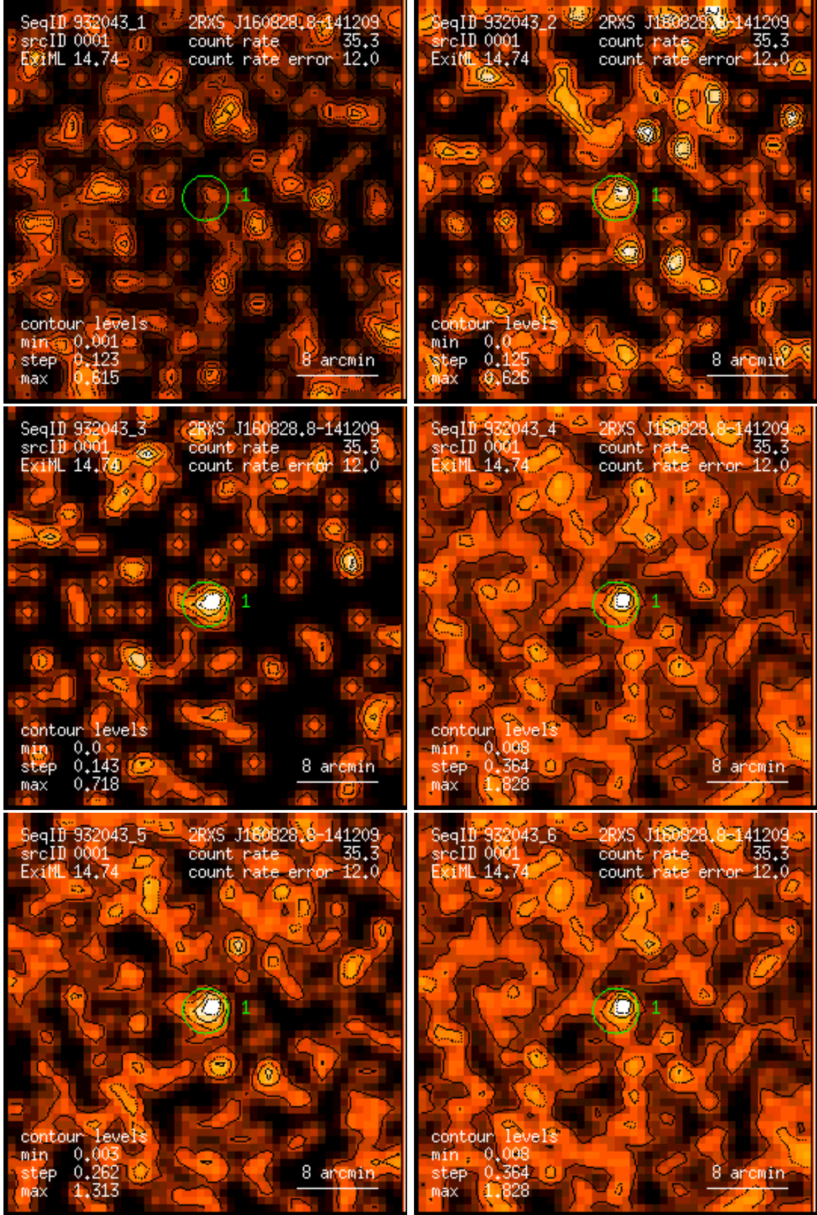
Figure 1: RASS 932043: detection 0001: band rate images, Gaussian filter: (1) PSPC channels 11 – 41, (2) 52 – 90, (3) 91 – 201, (4) 11 – 235, (5) 52 – 201, (6) 11 – 201. Broad band rates in counts/ks. Band rate contour levels in counts/ks/arcmin 2 .
