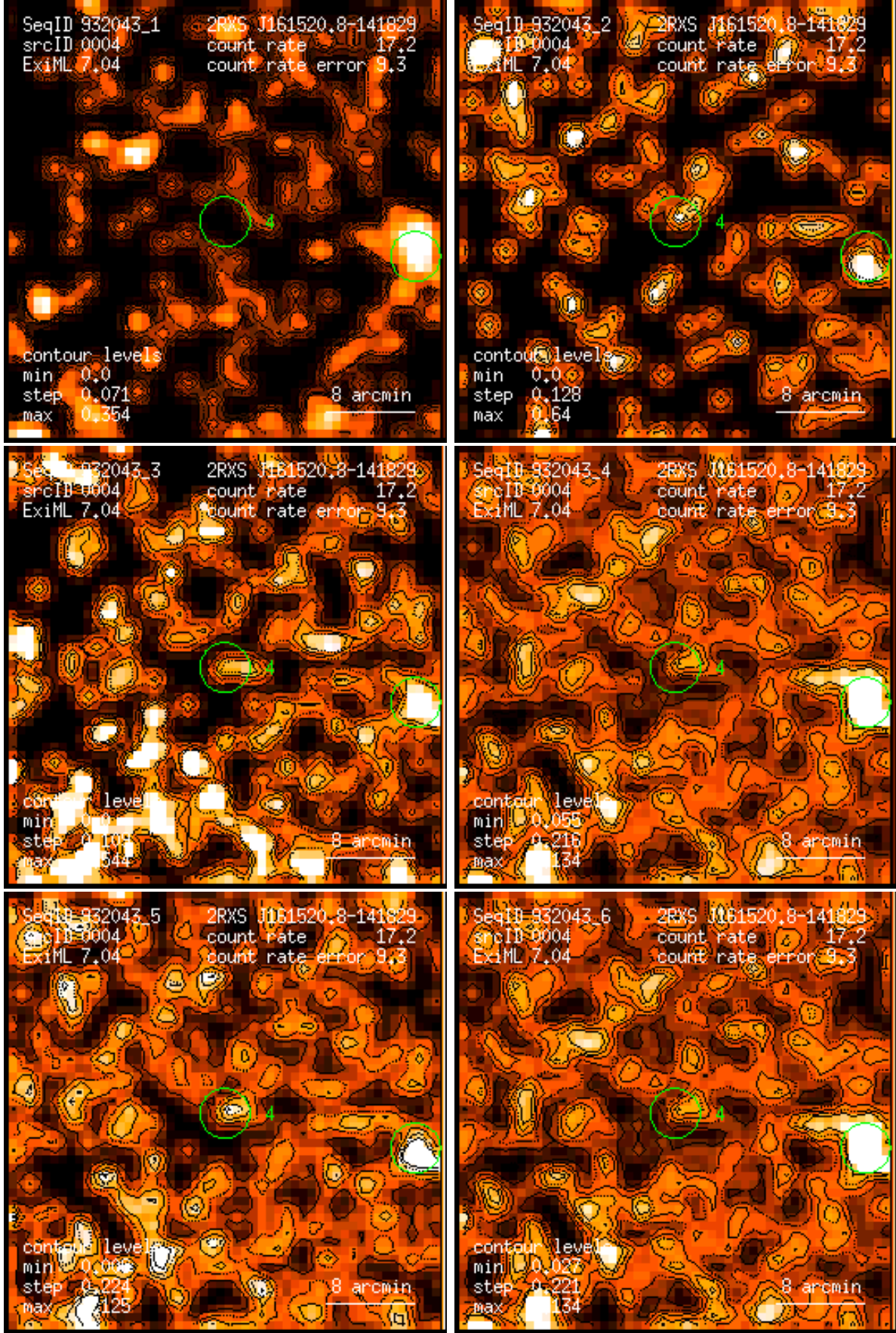
Figure 4: RASS 932043: detection 0004: band rate images, Gaussian filter: (1) PSPC channels 11 – 41, (2) 52 – 90, (3) 91 – 201, (4) 11 – 235, (5) 52 – 201, (6) 11 – 201. Broad band rates in counts/ks. Band rate contour levels in counts/ks/arcmin 2 .
