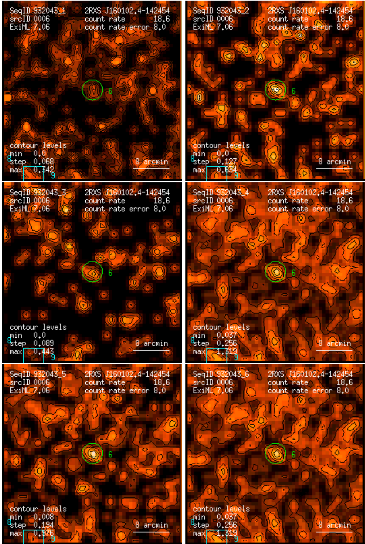
Figure 6: RASS 932043: detection 0006: band rate images, Gaussian filter: (1) PSPC channels 11 – 41, (2) 52 – 90, (3) 91 – 201, (4) 11 – 235, (5) 52 – 201, (6) 11 – 201. Broad band rates in counts/ks. Band rate contour levels in counts/ks/arcmin 2 .
