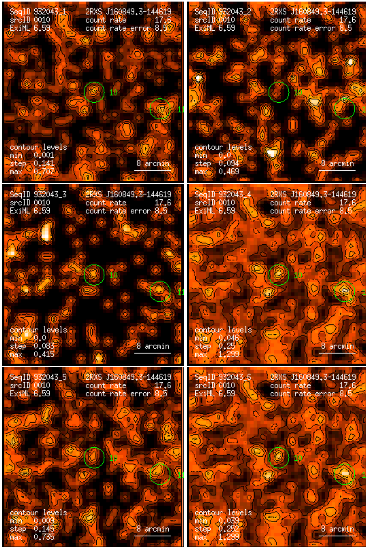
Figure 10: RASS 932043: detection 0010: band rate images, Gaussian filter: (1) PSPC channels 11 – 41, (2) 52 – 90, (3) 91 – 201, (4) 11 – 235, (5) 52 – 201, (6) 11 – 201. Broad band rates in counts/ks. Band rate contour levels in counts/ks/arcmin 2 .
