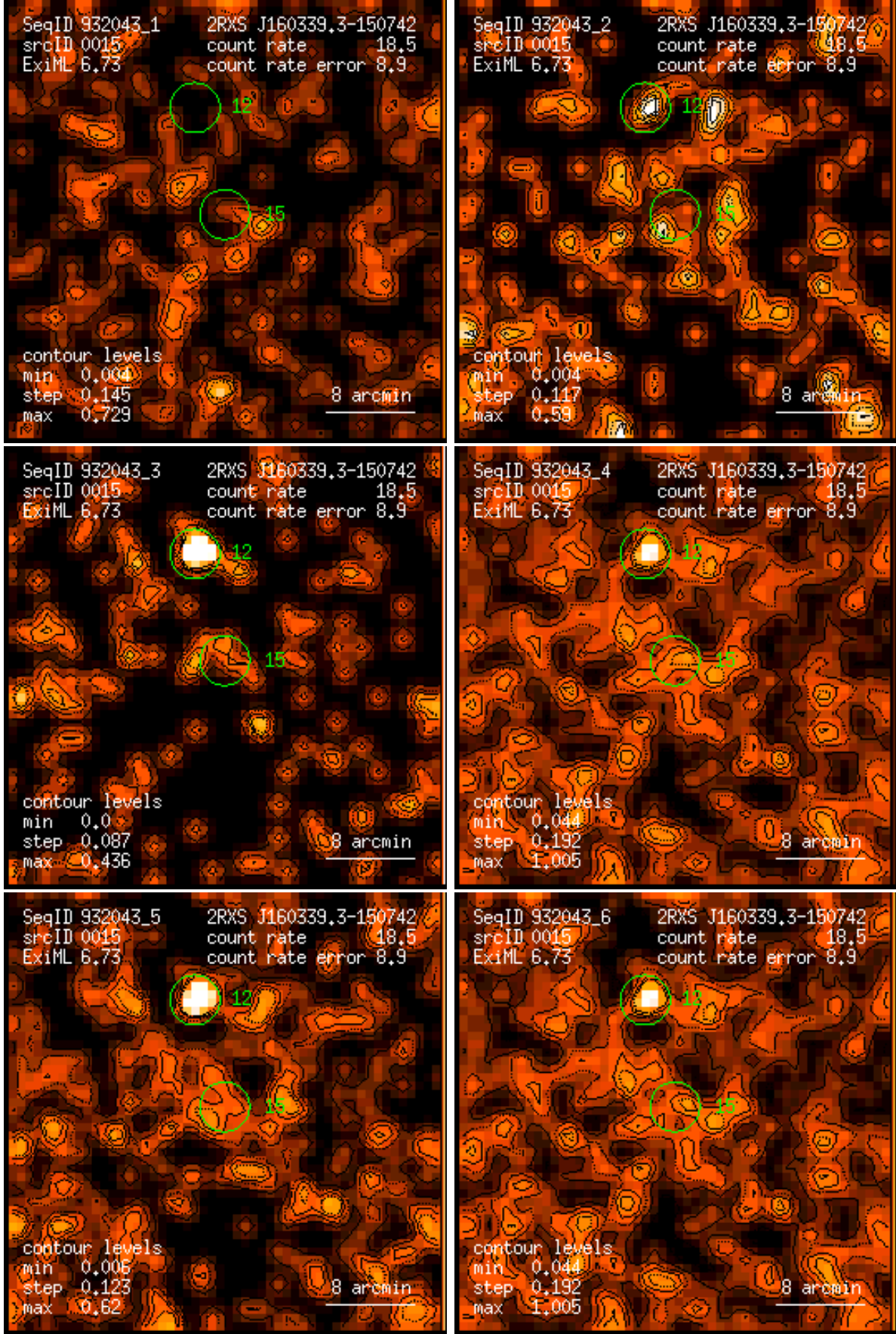
Figure 15: RASS 932043: detection 0015: band rate images, Gaussian filter: (1) PSPC channels 11 – 41, (2) 52 – 90, (3) 91 – 201, (4) 11 – 235, (5) 52 – 201, (6) 11 – 201. Broad band rates in counts/ks. Band rate contour levels in counts/ks/arcmin 2 .
