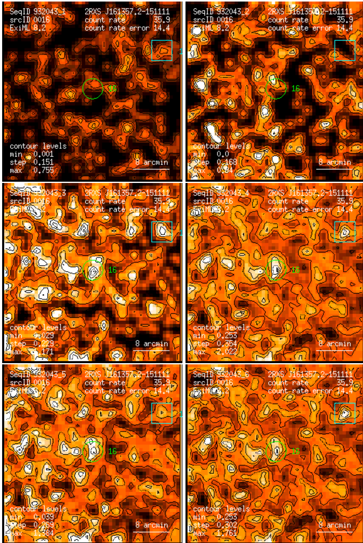
Figure 16: RASS 932043: detection 0016: band rate images, Gaussian filter: (1) PSPC channels 11 – 41, (2) 52 – 90, (3) 91 – 201, (4) 11 – 235, (5) 52 – 201, (6) 11 – 201. Broad band rates in counts/ks. Band rate contour levels in counts/ks/arcmin 2 .
