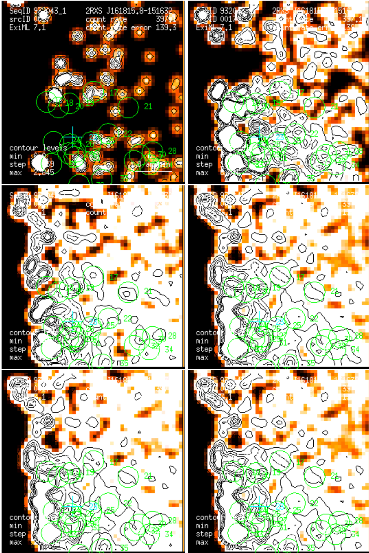
Figure 17: RASS 932043: detection 0017: band rate images, Gaussian filter: (1) PSPC channels 11 – 41, (2) 52 – 90, (3) 91 – 201, (4) 11 – 235, (5) 52 – 201, (6) 11 – 201. Broad band rates in counts/ks. Band rate contour levels in counts/ks/arcmin 2 .
