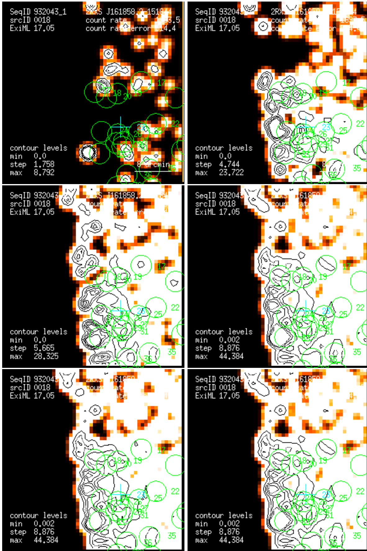
Figure 18: RASS 932043: detection 0018: band rate images, Gaussian filter: (1) PSPC channels 11 – 41, (2) 52 – 90, (3) 91 – 201, (4) 11 – 235, (5) 52 – 201, (6) 11 – 201. Broad band rates in counts/ks. Band rate contour levels in counts/ks/arcmin 2 .
