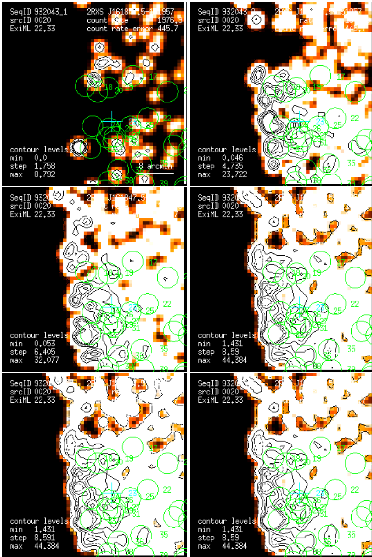
Figure 20: RASS 932043: detection 0020: band rate images, Gaussian filter: (1) PSPC channels 11 – 41, (2) 52 – 90, (3) 91 – 201, (4) 11 – 235, (5) 52 – 201, (6) 11 – 201. Broad band rates in counts/ks. Band rate contour levels in counts/ks/arcmin 2 .
