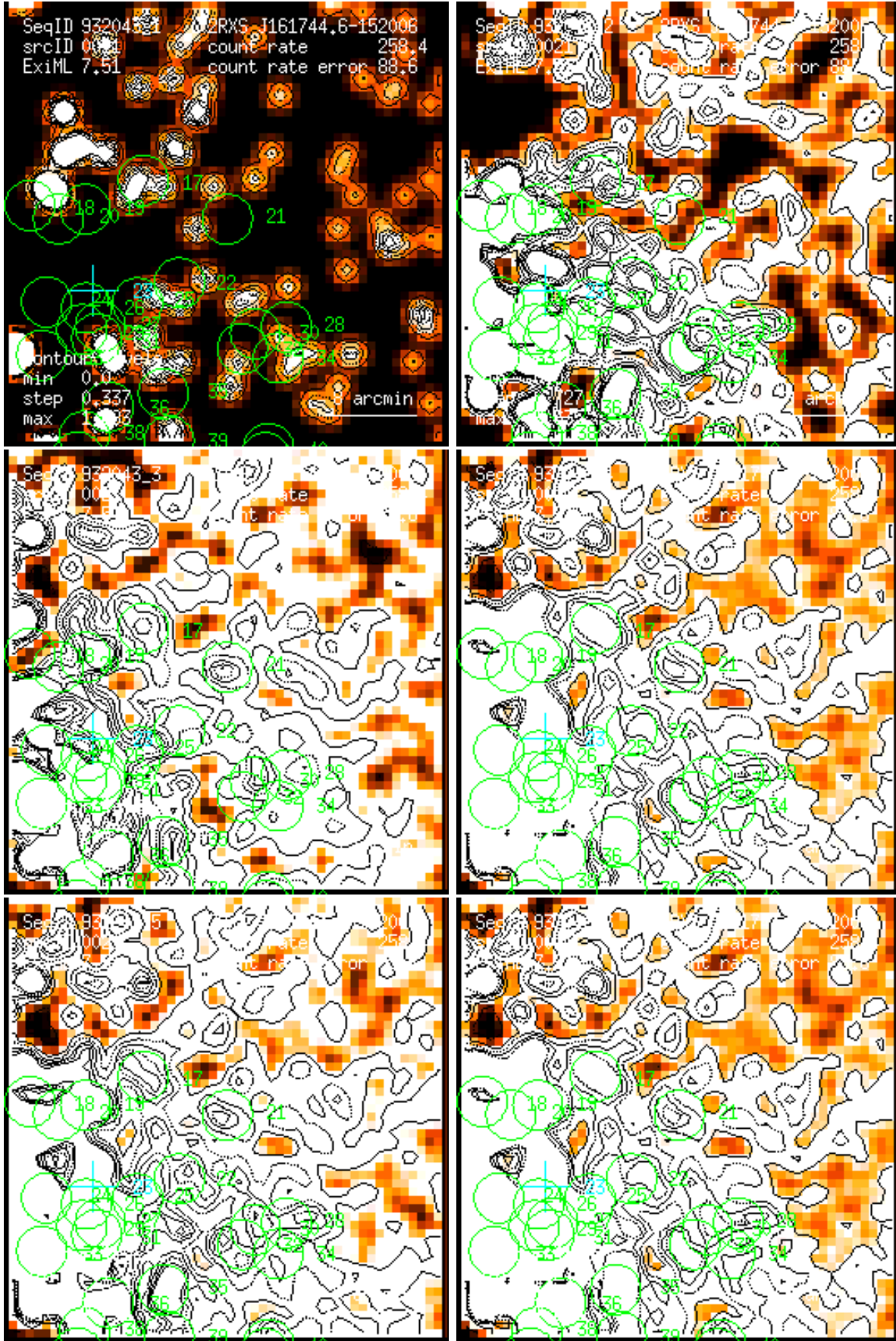
Figure 21: RASS 932043: detection 0021: band rate images, Gaussian filter: (1) PSPC channels 11 – 41, (2) 52 – 90, (3) 91 – 201, (4) 11 – 235, (5) 52 – 201, (6) 11 – 201. Broad band rates in counts/ks. Band rate contour levels in counts/ks/arcmin 2 .
