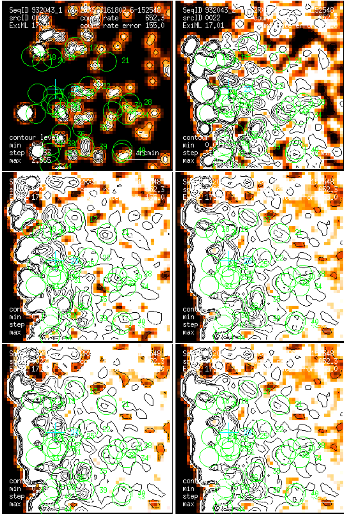
Figure 22: RASS 932043: detection 0022: band rate images, Gaussian filter: (1) PSPC channels 11 – 41, (2) 52 – 90, (3) 91 – 201, (4) 11 – 235, (5) 52 – 201, (6) 11 – 201. Broad band rates in counts/ks. Band rate contour levels in counts/ks/arcmin 2 .
