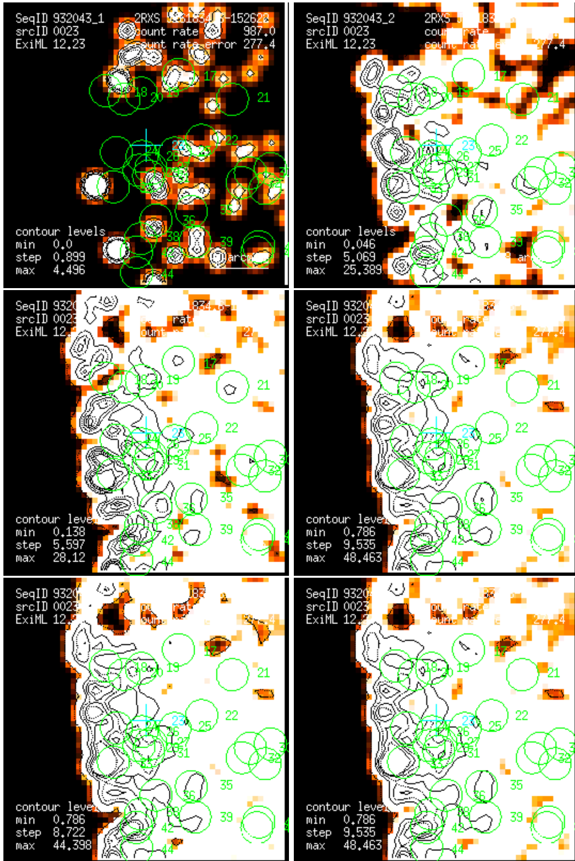
Figure 23: RASS 932043: detection 0023: band rate images, Gaussian filter: (1) PSPC channels 11 – 41, (2) 52 – 90, (3) 91 – 201, (4) 11 – 235, (5) 52 – 201, (6) 11 – 201. Broad band rates in counts/ks. Band rate contour levels in counts/ks/arcmin 2 .
