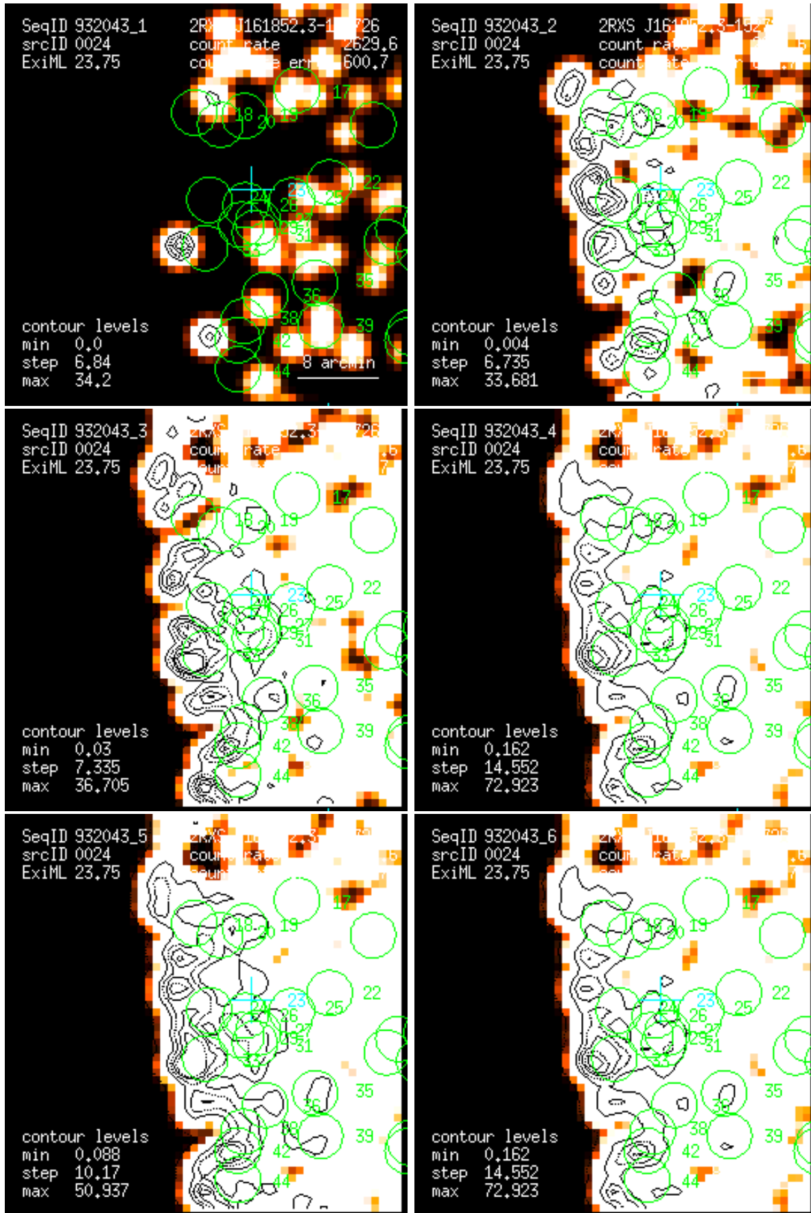
Figure 24: RASS 932043: detection 0024: band rate images, Gaussian filter: (1) PSPC channels 11 – 41, (2) 52 – 90, (3) 91 – 201, (4) 11 – 235, (5) 52 – 201, (6) 11 – 201. Broad band rates in counts/ks. Band rate contour levels in counts/ks/arcmin 2 .
