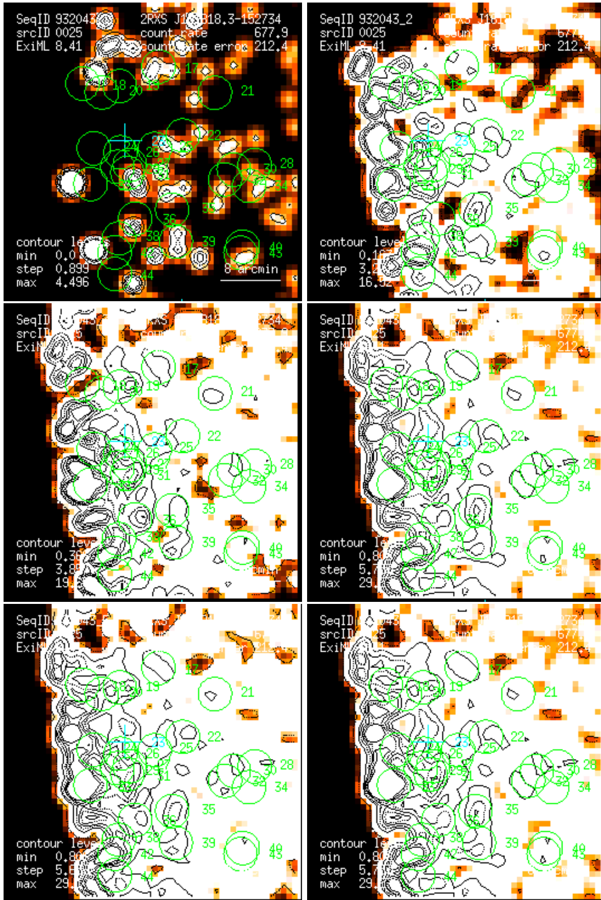
Figure 25: RASS 932043: detection 0025: band rate images, Gaussian filter: (1) PSPC channels 11 – 41, (2) 52 – 90, (3) 91 – 201, (4) 11 – 235, (5) 52 – 201, (6) 11 – 201. Broad band rates in counts/ks. Band rate contour levels in counts/ks/arcmin 2 .
