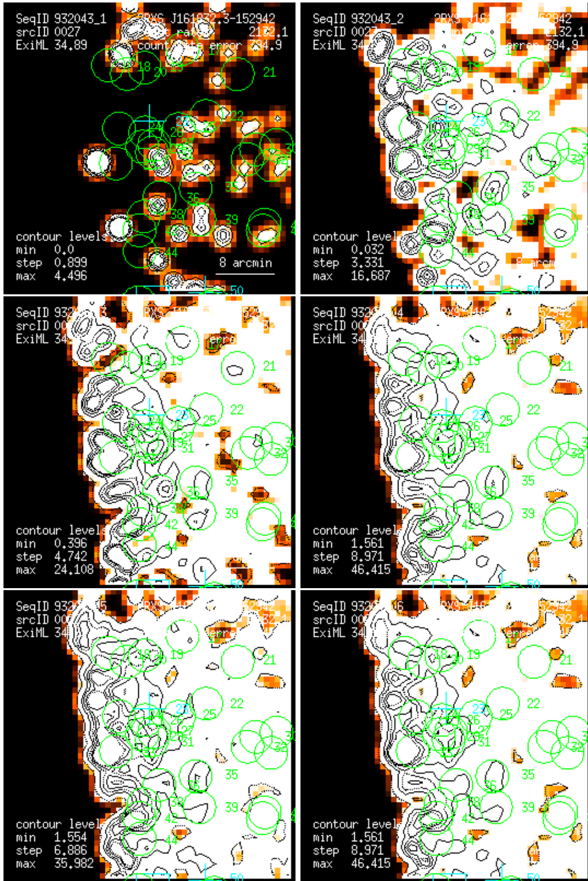
Figure 27: RASS 932043: detection 0027: band rate images, Gaussian filter: (1) PSPC channels 11 – 41, (2) 52 – 90, (3) 91 – 201, (4) 11 – 235, (5) 52 – 201, (6) 11 – 201. Broad band rates in counts/ks. Band rate contour levels in counts/ks/arcmin 2 .
