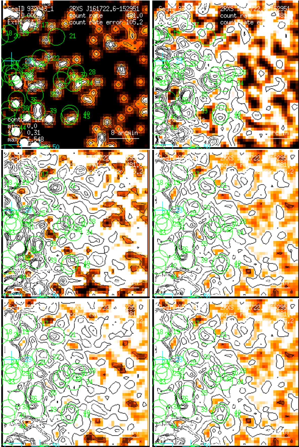
Figure 28: RASS 932043: detection 0028: band rate images, Gaussian filter: (1) PSPC channels 11 – 41, (2) 52 – 90, (3) 91 – 201, (4) 11 – 235, (5) 52 – 201, (6) 11 – 201. Broad band rates in counts/ks. Band rate contour levels in counts/ks/arcmin 2 .
