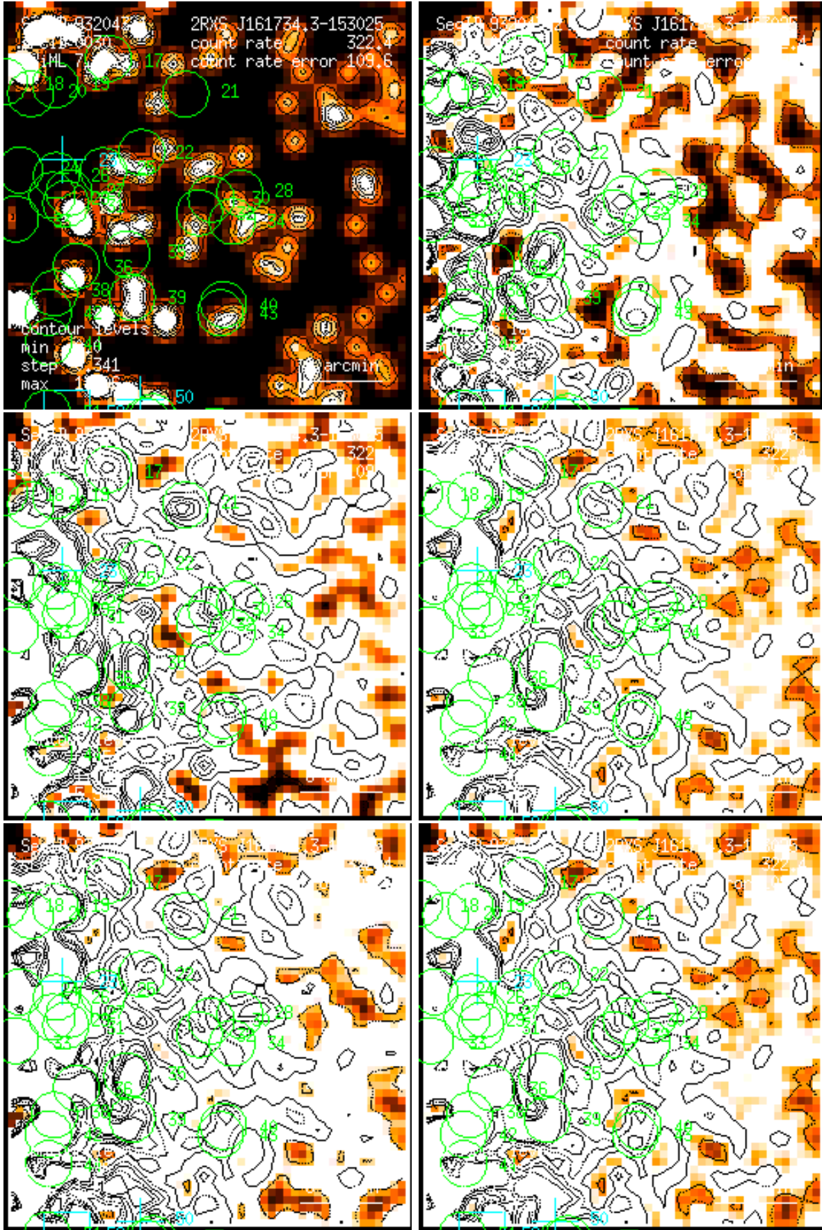
Figure 30: RASS 932043: detection 0030: band rate images, Gaussian filter: (1) PSPC channels 11 – 41, (2) 52 – 90, (3) 91 – 201, (4) 11 – 235, (5) 52 – 201, (6) 11 – 201. Broad band rates in counts/ks. Band rate contour levels in counts/ks/arcmin 2 .
