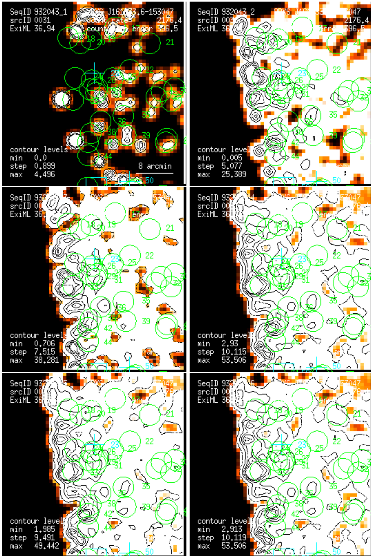
Figure 31: RASS 932043: detection 0031: band rate images, Gaussian filter: (1) PSPC channels 11 – 41, (2) 52 – 90, (3) 91 – 201, (4) 11 – 235, (5) 52 – 201, (6) 11 – 201. Broad band rates in counts/ks. Band rate contour levels in counts/ks/arcmin 2 .
