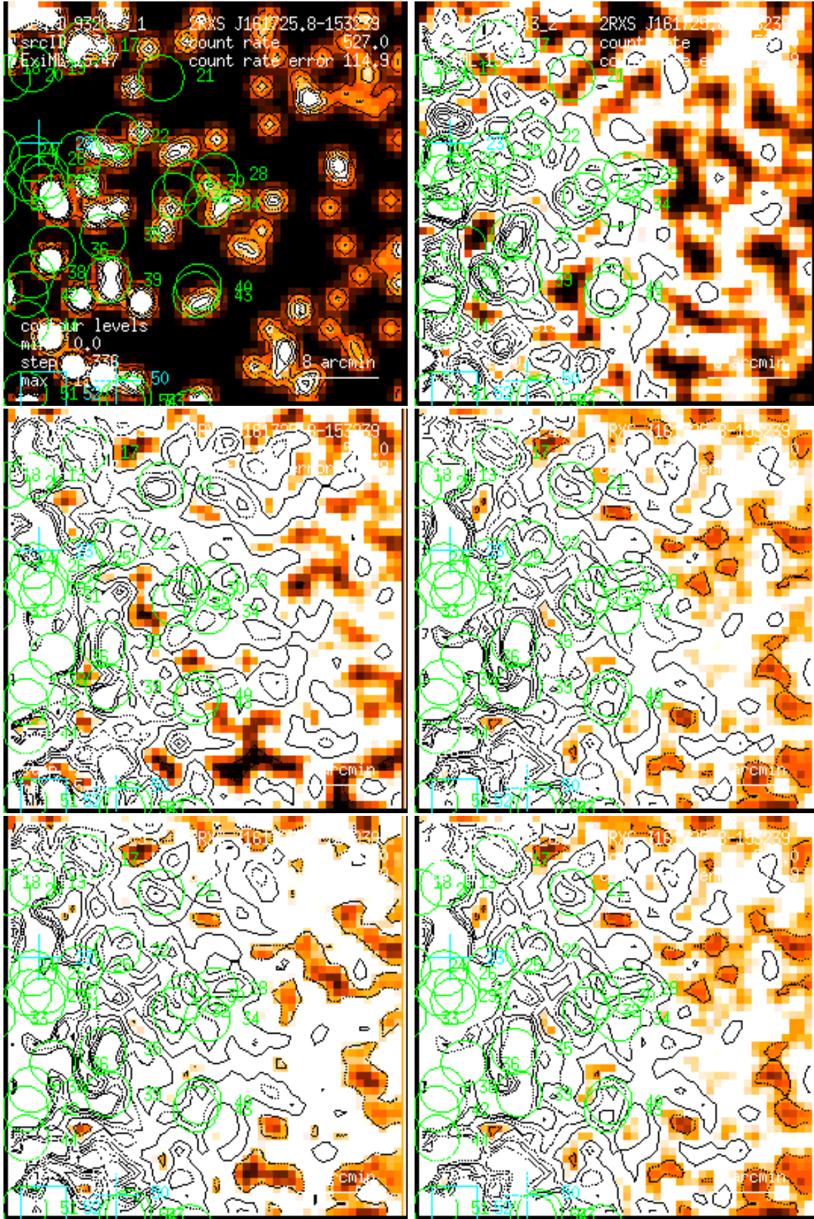
Figure 34: RASS 932043: detection 0034: band rate images, Gaussian filter: (1) PSPC channels 11 – 41, (2) 52 – 90, (3) 91 – 201, (4) 11 – 235, (5) 52 – 201, (6) 11 – 201. Broad band rates in counts/ks. Band rate contour levels in counts/ks/arcmin 2 .
