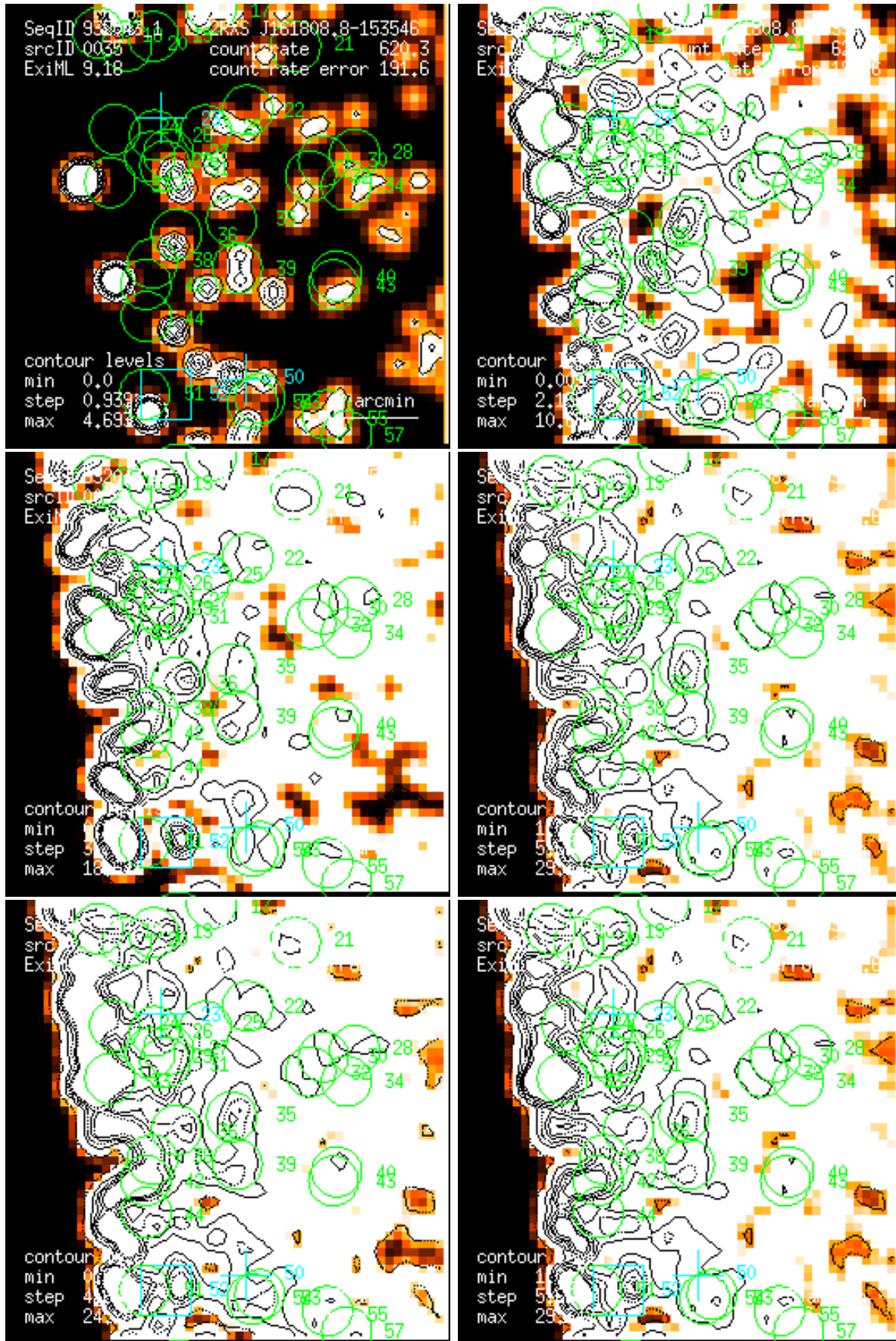
Figure 35: RASS 932043: detection 0035: band rate images, Gaussian filter: (1) PSPC channels 11 – 41, (2) 52 – 90, (3) 91 – 201, (4) 11 – 235, (5) 52 – 201, (6) 11 – 201. Broad band rates in counts/ks. Band rate contour levels in counts/ks/arcmin 2 .
