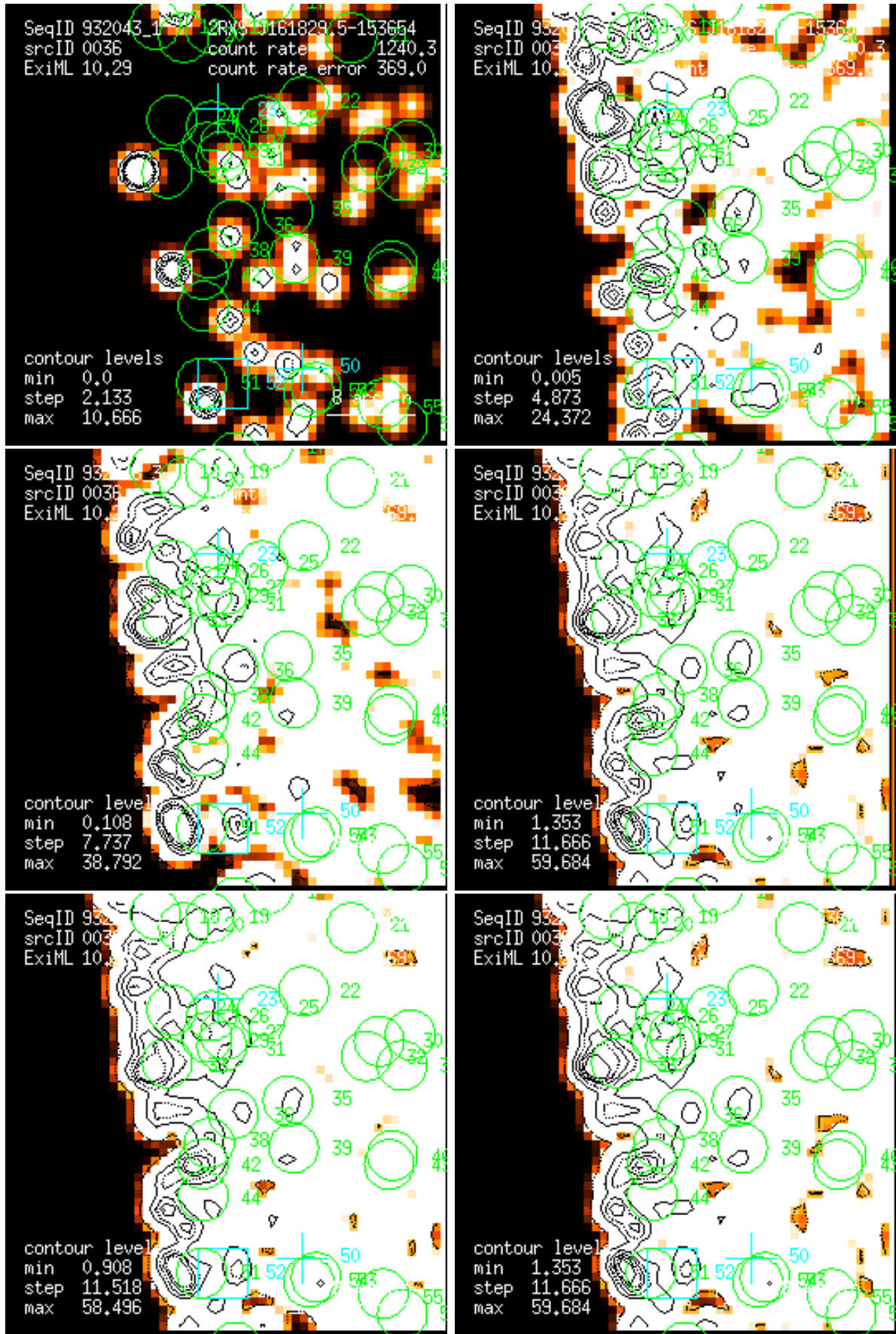
Figure 36: RASS 932043: detection 0036: band rate images, Gaussian filter: (1) PSPC channels 11 – 41, (2) 52 – 90, (3) 91 – 201, (4) 11 – 235, (5) 52 – 201, (6) 11 – 201. Broad band rates in counts/ks. Band rate contour levels in counts/ks/arcmin 2 .
