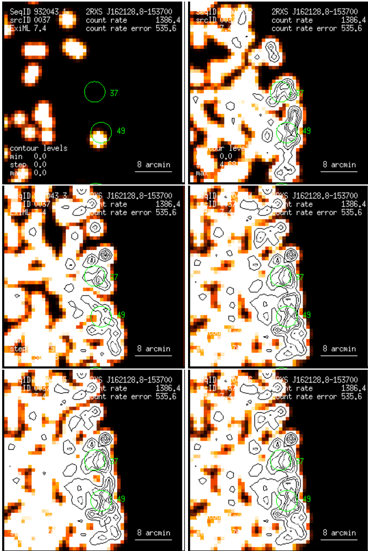
Figure 37: RASS 932043: detection 0037: band rate images, Gaussian filter: (1) PSPC channels 11 – 41, (2) 52 – 90, (3) 91 – 201, (4) 11 – 235, (5) 52 – 201, (6) 11 – 201. Broad band rates in counts/ks. Band rate contour levels in counts/ks/arcmin 2 .
