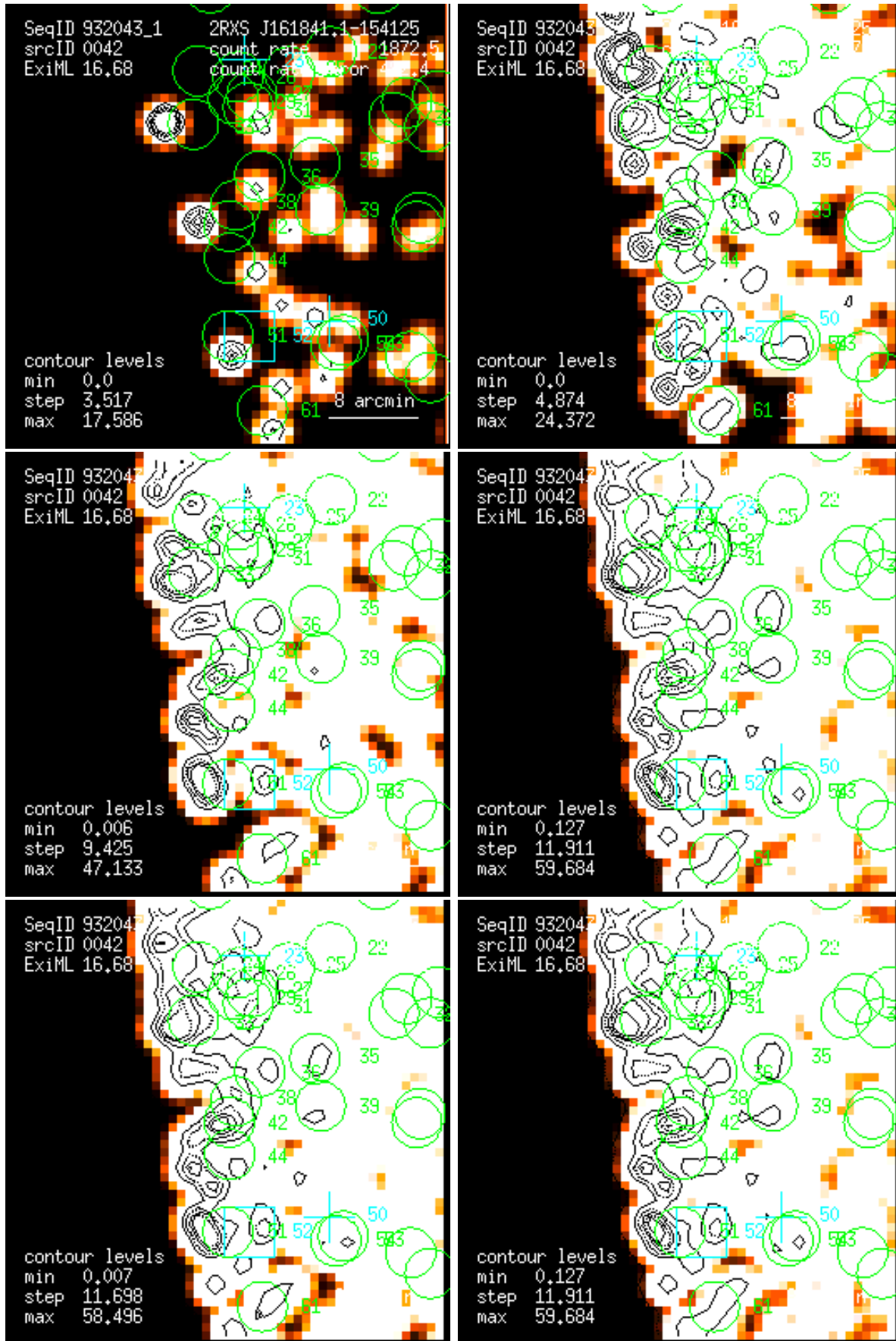
Figure 42: RASS 932043: detection 0042: band rate images, Gaussian filter: (1) PSPC channels 11 – 41, (2) 52 – 90, (3) 91 – 201, (4) 11 – 235, (5) 52 – 201, (6) 11 – 201. Broad band rates in counts/ks. Band rate contour levels in counts/ks/arcmin 2 .
