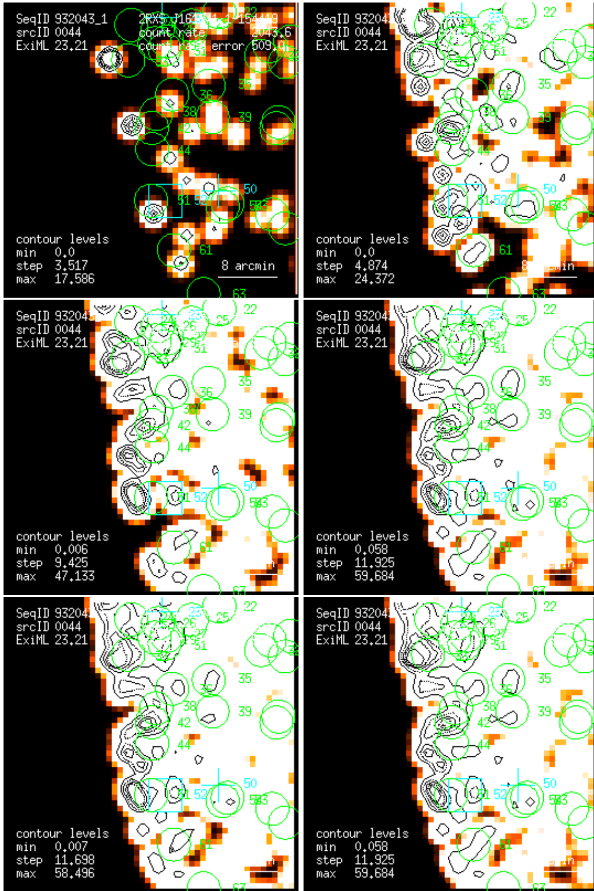
Figure 44: RASS 932043: detection 0044: band rate images, Gaussian filter: (1) PSPC channels 11 – 41, (2) 52 – 90, (3) 91 – 201, (4) 11 – 235, (5) 52 – 201, (6) 11 – 201. Broad band rates in counts/ks. Band rate contour levels in counts/ks/arcmin 2 .
