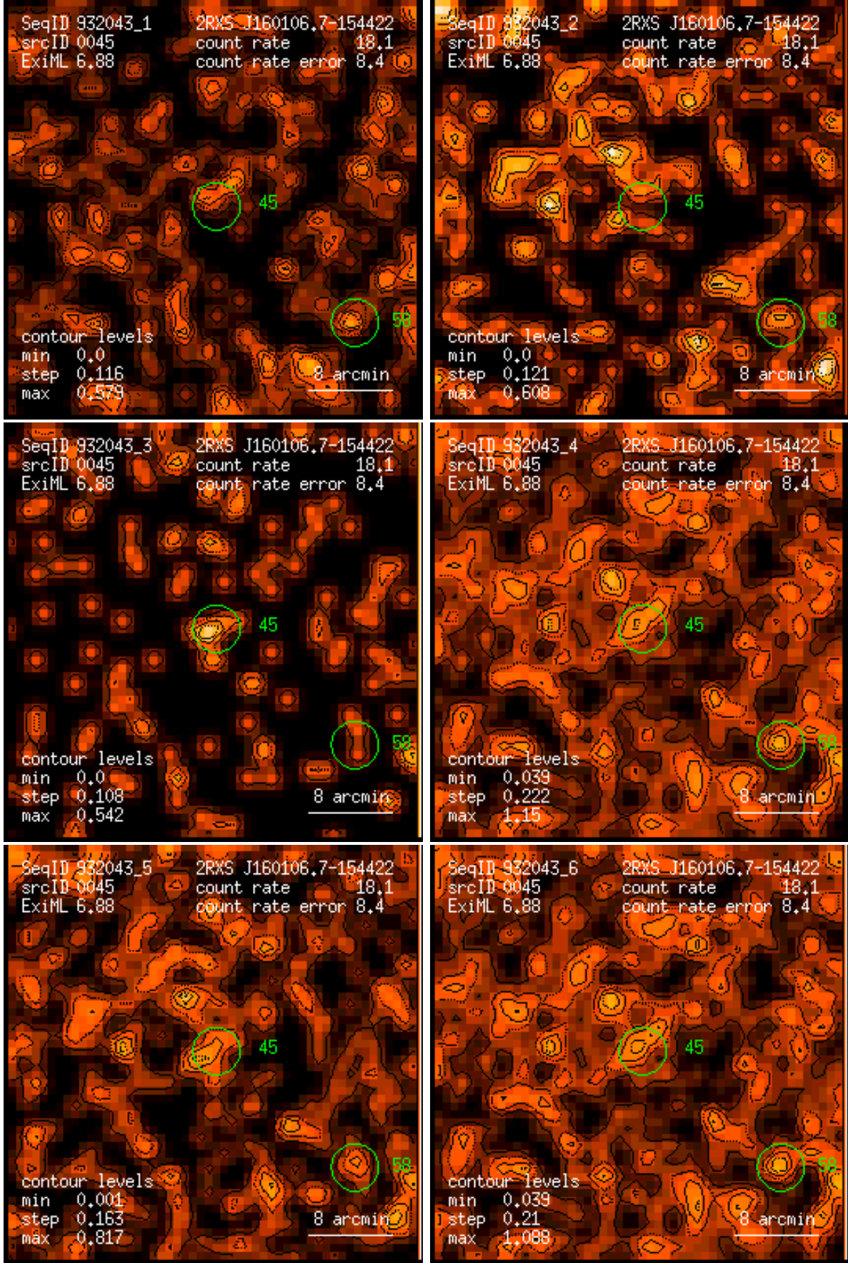
Figure 45: RASS 932043: detection 0045: band rate images, Gaussian filter: (1) PSPC channels 11 – 41, (2) 52 – 90, (3) 91 – 201, (4) 11 – 235, (5) 52 – 201, (6) 11 – 201. Broad band rates in counts/ks. Band rate contour levels in counts/ks/arcmin 2 .
